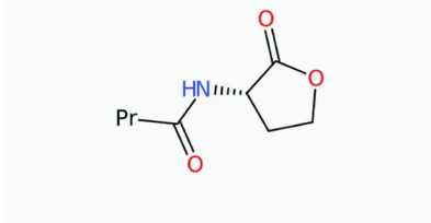
C4-HSL
