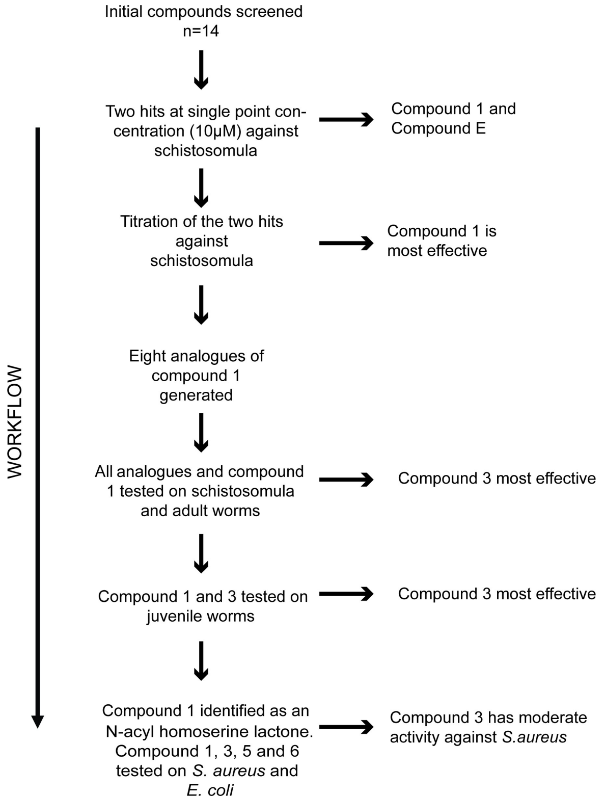
Fig 1. The screening pipeline utilised in this anti-infective study. A total of 14 compounds were initially screened against S. mansoni schistosomula at a final concentration of 10 \mu M. Hits were subsequently subjected to dose response titrations with the most effective anti-schistosomula compound (Compound 1) subsequently being used as a template for the preparation of further derivatives (compounds 2–9). Compounds 2–9 were subsequently subjected to dose response titrations against schistosomula and adult worms. The most
