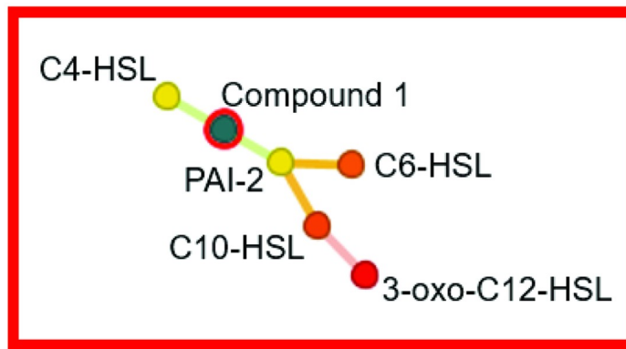
Compound 1
