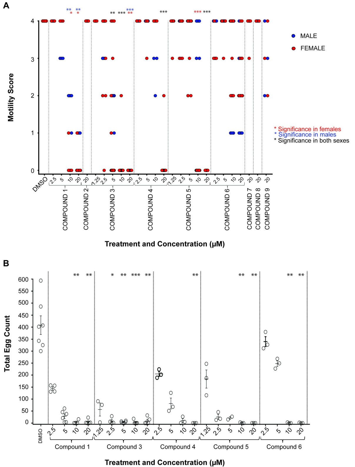
Fig 3. Adult schistosome motility and egg production are differentially affected by the nine N-acyl homoserine lactones. A) Adult S. mansoni worm pairs were cultured in decreasing compound concentrations of between 20 \mu\text{M} and 1.25 \mu\text{M} (not all concentrations were used for all compounds) for 72 hrs at 37°C, 5% CO 2 . Parasite motility was evaluated for each sex and scored using the WHO-TDR scoring
