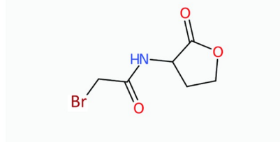
Compound 1
