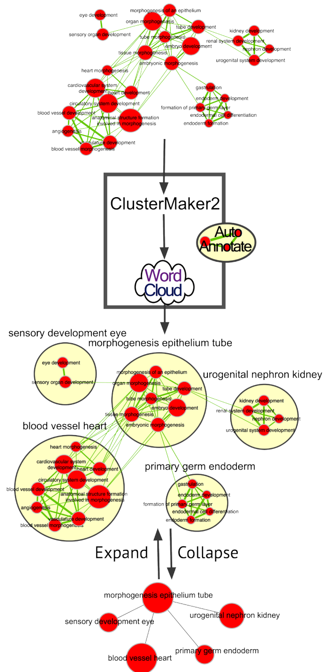
Figure 1. AutoAnnotate overview. A network is clustered, textual annotation associated with each cluster is automatically summarized as a single cluster label, and the results are visualized. Users can customize the view by selectively collapsing and expanding clusters.
