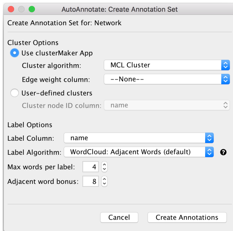
Figure 2. The Create Annotation Set dialog. Cluster options: ClusterMaker2 requires a clustering algorithm and edge weight attribute to be selected, otherwise a node attribute must be selected. Label options: User selects the node attribute to use for creating labels, the labelling algorithm to use, and the maximum number of words per label.
