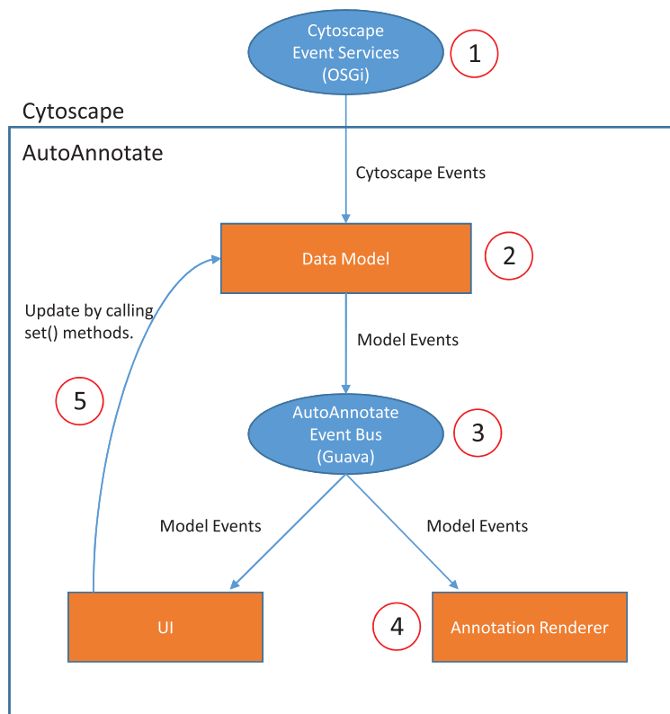
Figure 5. Event Flow. 1) Cytoscape events are fired using OSGi services (e.g. SetCurrentNetworkViewEvent, NetworkViewAboutToBeDestroyedEvent). 2) The AutoAnnotate Model Manager reacts to Cytoscape events and updates the Data Model. 3) The ModelManager fires Model Events over the Guava EventBus (e.g. AnnotationSetAddedEvent, ClusterAddedEvent). 4) The UI and Annotation Renderer modules each respond to a subset of the model events. There is no direct dependency between the UI and the Annotation Renderer. 5) The UI directly updates the Model, which causes Model Events to fire, which updates the UI and Annotations.
