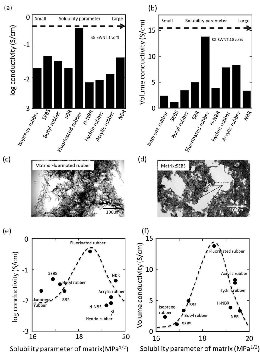
Figure 1 | (a,b) Volume conductivities of various rubber composites containing 1(a) and 10vol%(b) SG-SWCNT. (c,d) Optical micrographs of SG-SWCNT morphology in fluorinated rubber (c) and SEBS(d). Ultrathin sections are prepared with cryo-microtoming. Black region is SG-SWCNT and transparent region is rubber.
