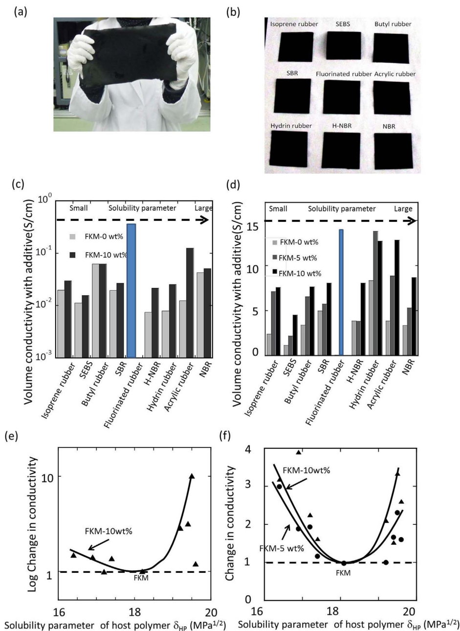
Figure 4 | (a, b) Photograph showing an A4 scale SG-SWCNT/fluorinated rubber (10 vol%)/isoprene-rubber composite (a) and SG-SWCNT/elastomers with fluorinated rubber as additive (b). (c,d) Volume conductivity change with adding 5 and 10 wt% fluorinated rubber. (c) and (d) indicate 1 and 10 vol% SG-SWCNT, respectively. (e, f) Change in conductivities (conductivity with fluorinated rubber divided by conductivity without fluorinated rubber) versus solubility parameter of host polymer.
