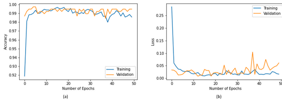
Fig. 6. Performance of the binary classifier of COV-VGX. (a) Training and validation accuracy and (b) Training and validation loss.
