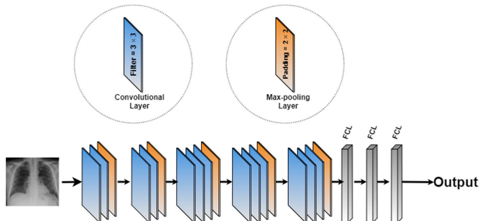
Fig. 3. VGG-16 architecture.
