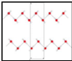
Fig. 3. One-dimensional supramolecular chain made up of water molecules.
