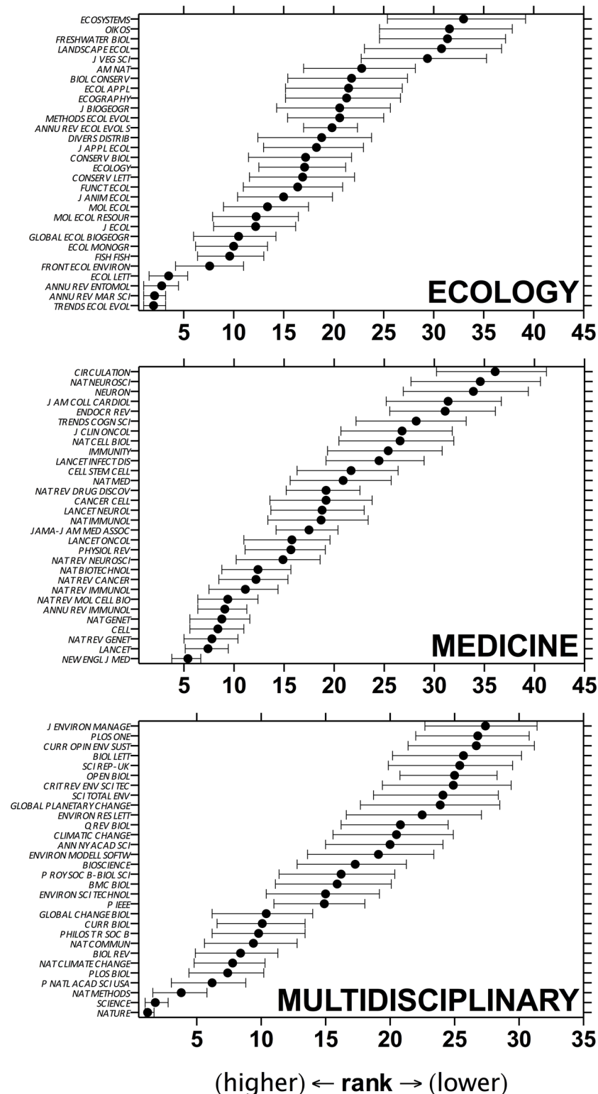
Fig 1. Mean rank (± 95% uncertainty limits) of the top 30 journals for two disparate biological disciplines: Ecology and Medicine, plus one Multidisciplinary theme. Journals are ordered by mean rank of five metrics: IF, IM, SNIP, SJR and h5/\log_{10}(n) ; statistics were estimated using \kappa -resampling with 10,000 iterations, from a total sample of 100 journals for Ecology and Medicine and 50 journals for Multidisciplinary (see main text for details). Journal abbreviations follow the Web of Science standard.
