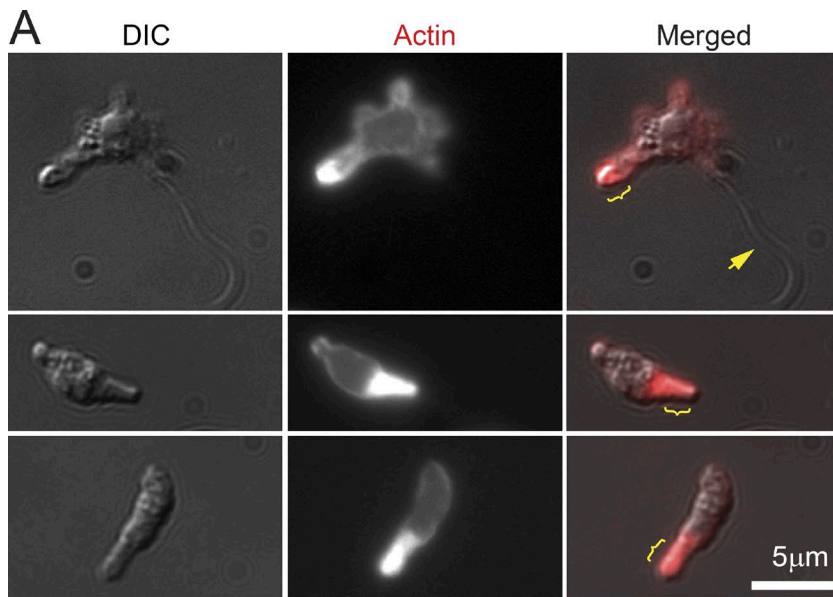
Figure 6. Chytrid pseudopods are actin filled and require both actin polymerization and Arp2/3 activity. (A) Fixed chytrid cells with and without a flagellum (arrow). Staining with fluorescent phalloidin reveals a thin shell of cortical actin surrounding the cell body and a dense network of polymerized actin filling the pseudopods (brackets). DIC, differential interference contrast. (B) Two examples of chytrid cells with pseudopods that lose them when treated with 10 nM latrunculin B, an inhibitor of actin polymerization. Dynamic pseudopods (brackets) return after drug washout. (C) Quantification of reversible inhibition of pseudopods by latrunculin B (Lat B). Only cells that were making pseudopods before treatment and that were not washed away during the experiment were counted. (D) Two examples of chytrid cells with pseudopods that lose them when treated with 10 \mu M CK-666, an inhibitor of Arp2/3 activity. Pseudopods return after drug washout. (E) Quantification of reversible inhibition of pseudopods by CK-666. Only cells that were making pseudopods before treatment and that were not washed away during the experiment were counted. Symbols are means from three biological replicates, each with at least 29 (C) or 17 (E) cells. P-values were obtained from two-tailed paired t tests.
