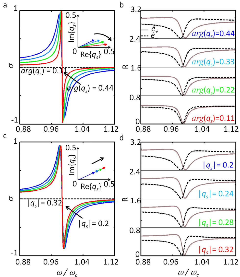
Figure 4. Optical spin-density and reflection spectra as a function of (a,b) chirality i.e. arg(q_s) = 0.44 to 0.11 and (c,d) birefringence i.e. |q_s| = 0.2 to 0.32 . In (b,d) the \hat{e}_+ (solid) and \hat{e}_- (dashed) lines represent the states of spin-density \sigma = +1 and -1 , respectively.
