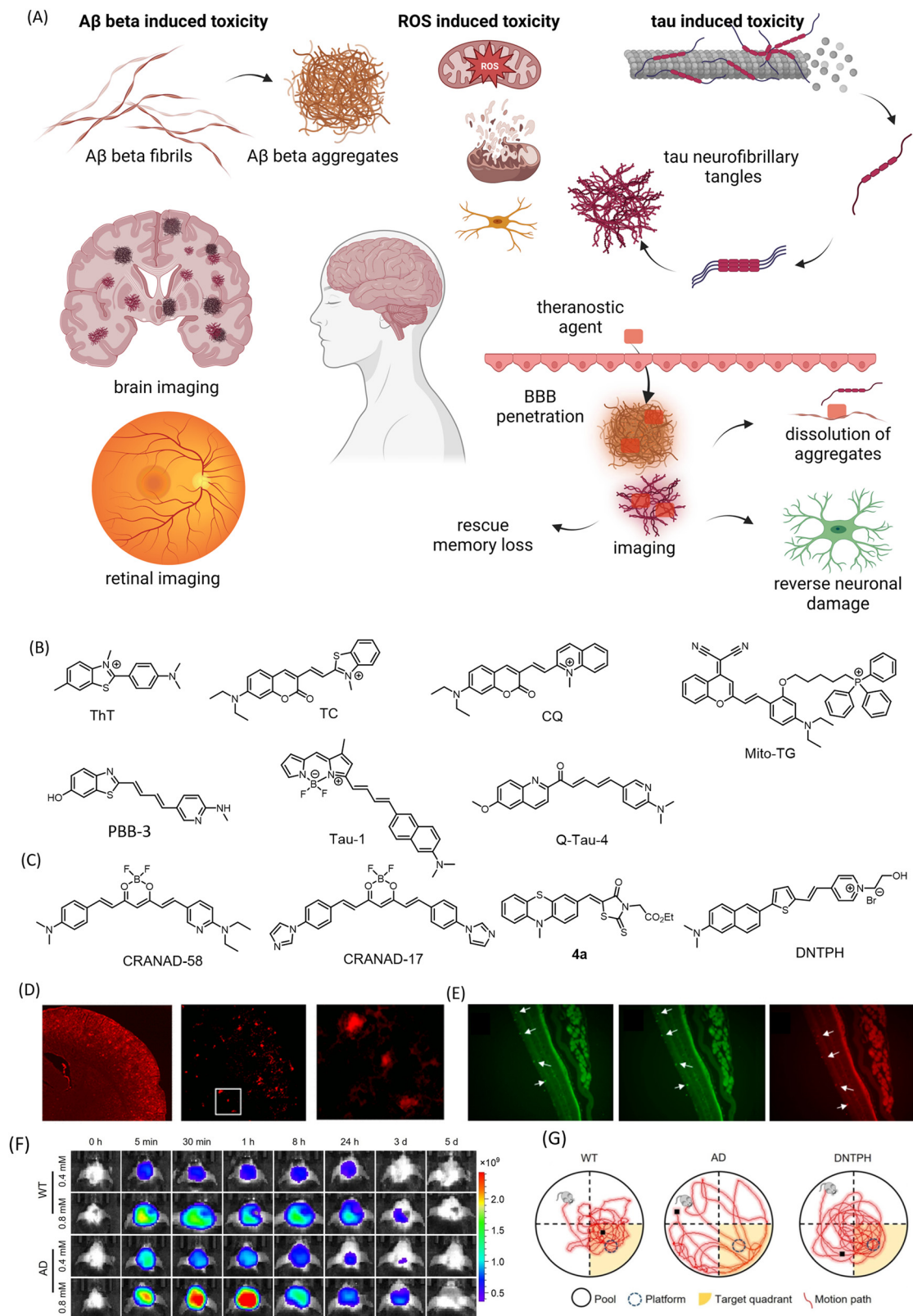
Fig. 10 (A) Multifaceted toxicity, diagnosis, and treatment strategies in Alzheimer's disease. (B) turn-on fluorescent probes for A \beta (ThT, TC, and CQ), mitochondria (Mito-TG) and tau (PBB-3, Tau-1, Q-Tau-4, 2e ) aggregates. (C) Molecular structures of theranostic candidates for Alzheimer's disease. (D) Fluorescence images of brain slices from 18 months old APP/PS1 mice stained with CRANAD-58. Reproduced from ref. 119 with permission from American Chemical Society, copyright 2013. (E) Fluorescence images of retinal tissue slices stained with ThT, A \beta antibody ab2454, and 4a1 in double Tg mice. Reproduced from ref. 120 with permission from American Chemical Society, copyright 2017. (F) In vivo fluorescence imaging of wild type (WT) and AD mice brain (7 months old) treated with DNTPH and (G) representative swimming track showing improvement in recognition/cognitive ability in AD mice treated with DNTPH, evident from Morris water maze (MWM) test. (F) and (G) Are reproduced from ref. 122 with permission from Wiley-VCH, copyright 2023. (A) Was created using https://BioRender.com .
