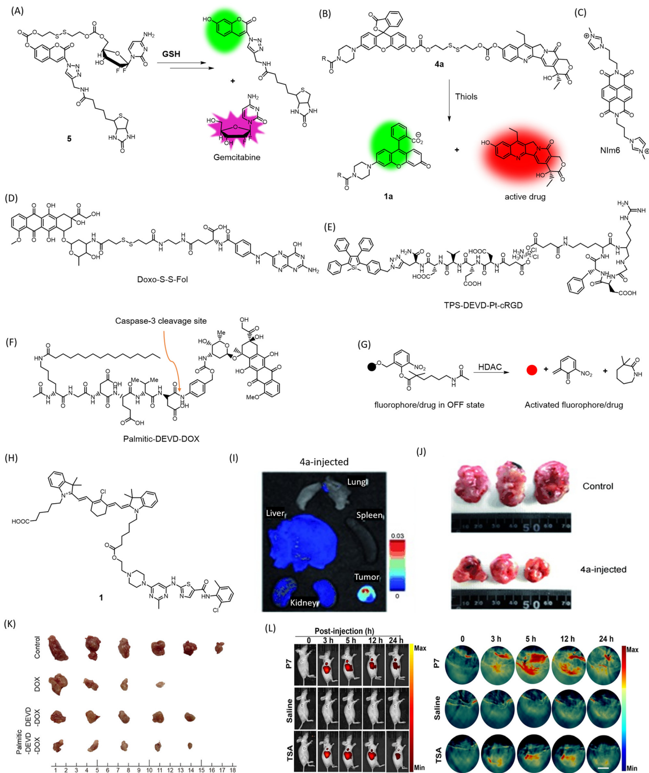
Fig. 4 Mechanism of cleavage of (A) 5 and (B) 4a by GSH to release fluorophore and the drug Gemcitabine and SN-38 respectively, structures of (C) Nlm6, (D) Doxo-S-S-Fol, (E) TPS-DEVD-Pt-cRGD, (F) Palmitic-DEVD-DOX, (G) mechanism of HDAC-responsive cleavage of conjugate to activate the drug/fluorophore, (H) Structure of conjugate 1 , (I) ex vivo fluorescence imaging of organs to visualize preferential accumulation of 4a in tumor site (J) reduction in tumor volume in HeLa mice xenografts treated with 4a for 35 days. (I) and (J) Are reproduced from ref. 70 with permission from Wiley VCH, copyright 2014, (K) chemotherapeutic efficacy of Palmitic-DEVD-DOX conjugate in CT26 bearing mice in comparison to unconjugated counterparts. Reproduced from ref. 75 with permission from American Chemical Society, copyright 2023. (L) In vivo NIRF/PA imaging of MDA-MB-231 tumor-bearing mice administered with HDAC responsive P7 and HDAC inhibitor trichostatin A (TSA). Reproduced from ref. 76 with permission from Wiley VCH, copyright 2022.
