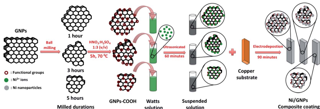
Fig. 1 Illustration of the fabrication process of GNPs reinforced nickel coating with the different GNPs size using the electrodeposition technique.
