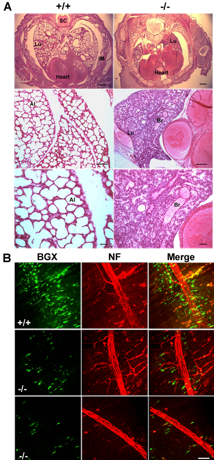
Figure 2. Cbx1 -/- neonates do not inflate their lungs, and E19 Cbx1 -/- embryos exhibit reduced clusters of postsynaptic AChRs within diaphragm muscle. (A) Hematoxylin and eosin–stained transverse sections through the midbody of wild-type (left) and Cbx1 -/- (right) neonates showing lack of inflation of the lungs in the Cbx1 -/- neonates. Al, alveolus; Br, bronchiole; IM, intercostal muscle; Lu, lung; SC, spinal cord. Bars: (top) 450 \mu m; (middle) 150 \mu m; (bottom) 50 \mu m. (B) Staining of E19 wild-type diaphragms (top) with antibodies to NF (red) shows that the diaphragm is clearly innervated. Bungarotoxin-positive (BGX; green) AChRs are clustered around the nerve and its branches. The clusters of bungarotoxin-positive AChRs are much reduced in E19 Cbx1 -/- diaphragms (middle and bottom), and, in some cases, the branching of the innervating nerve is also reduced (bottom; see red NF staining). Bar, 25 \mu m.
