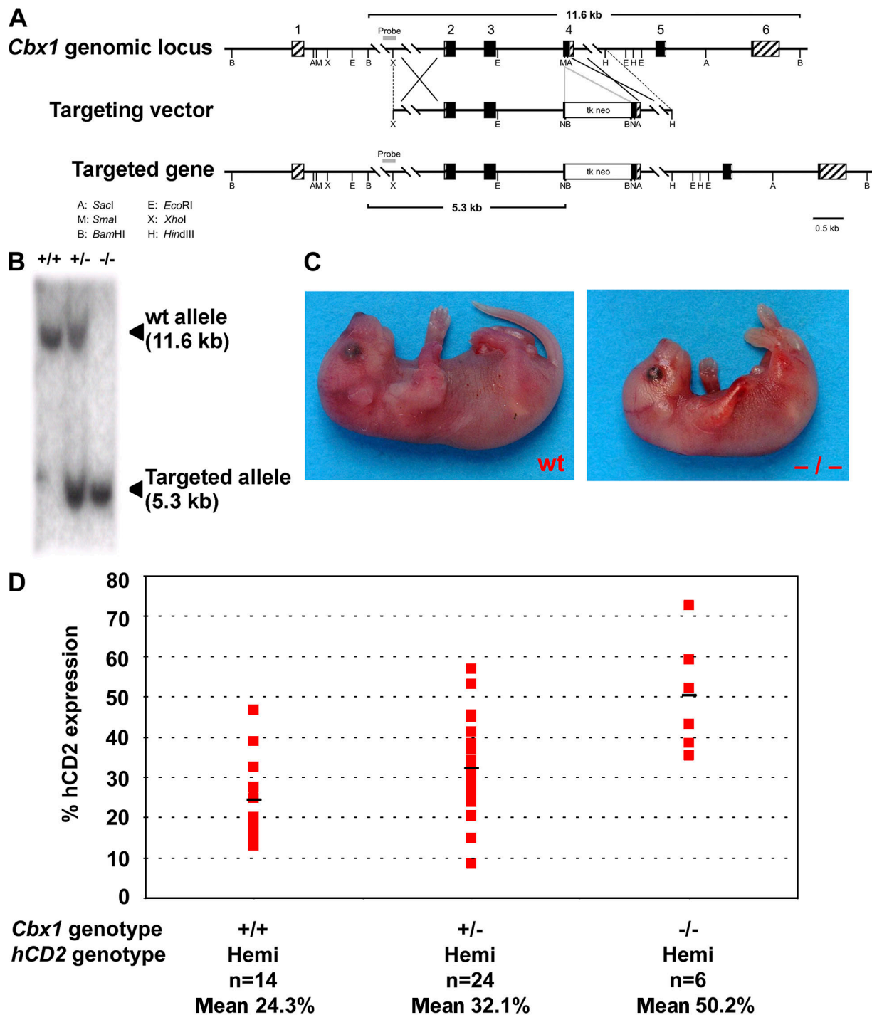
Figure 1. Cbx1 gene function is essential, and its product, HP1- \beta , is a modifier of PEV. (A) The relevant regions in the wild-type Cbx1 locus (top; see Materials and methods), the TK- Neo targeting vector (middle), and the targeted gene (bottom). Coding regions are depicted by closed boxes. Noncoding regions are denoted by striped boxes. The DNA probe used to screen for targeting events is shown as a shaded rectangle. (B) Southern blot authentication of germline transmission of the Cbx1 mutation. Bam HI digest of genomic DNA produces an 11.6-kb fragment for the wild-type (wt) allele and a diagnostic 5.3-kb fragment for the targeted allele. (C) Images of wild-type (left) and Cbx1 -/- (right) neonates. (D) Scatter plots showing the results of flow cytometry analysis of the proportion of transgenic embryonic DP (CD4 + CD8 + ) thymocytes that express hCD2 taken from the three Cbx1 genotypes. Each point represents the result from a single embryo. The mean expression of hCD2 in embryonic thymocytes from Cbx1 +/- animals is higher than that for Cbx1 +/+ animals, but not significantly. The mean expression of hCD2 in thymocytes taken from Cbx1 -/- animals is significantly different from expression in thymocytes taken from the parental genotypes ( P < 0.001 ). Black lines represent the means.
