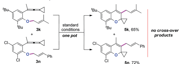
Scheme 4 Mechanistic experiments.
