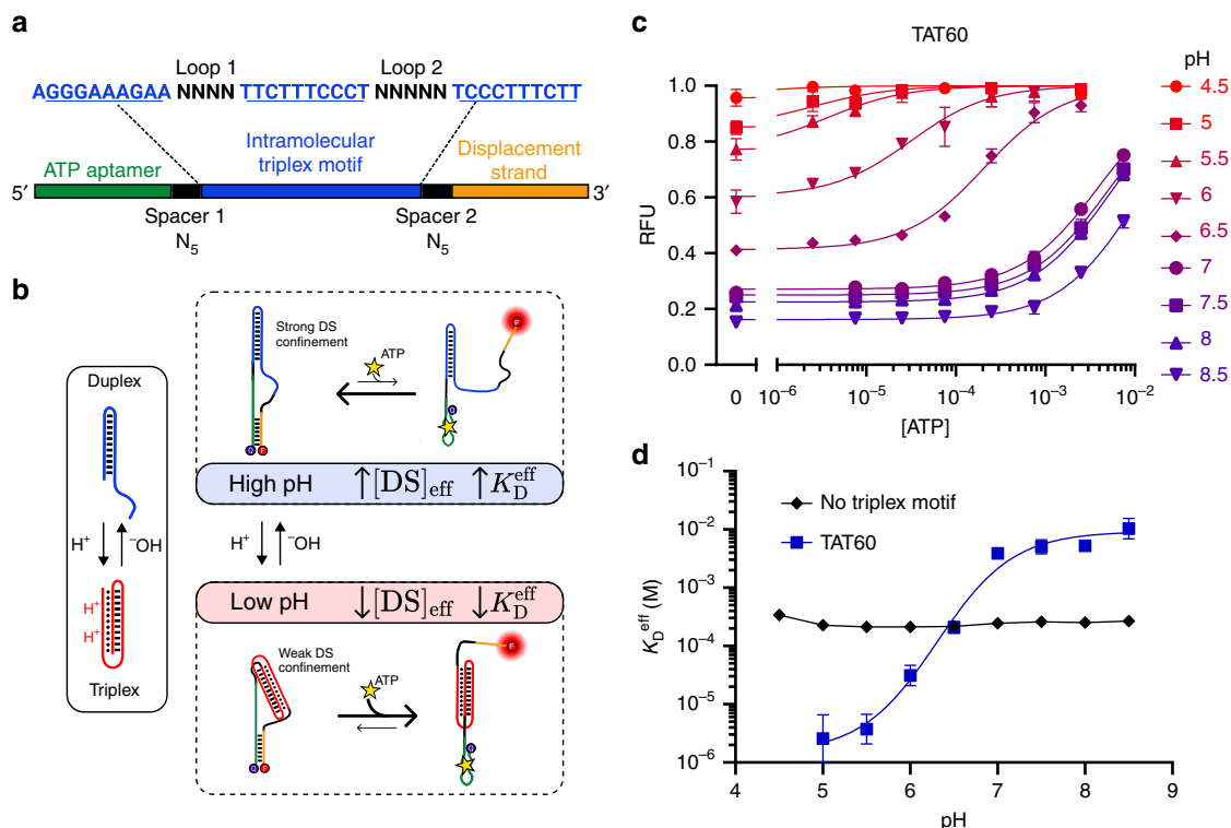
Fig. 1 Design of an ATP aptamer for selective binding at low pH. a An intramolecular triplex motif is inserted into the linker domain, which connects the ATP aptamer and displacement strand (DS). The unconstrained loop and spacer sequences are optimized to minimize interference with the aptamer secondary structure. The construct shown here is TAT60, reflecting the 60% TAT composition of the triplex motif. b A simplified model for pH-dependent binding. pH dependence is achieved via conformational changes in the triplex motif, which increase the effective DS concentration near the aptamer ( [DS]_{\text{eff}} ) at high pH, thereby inhibiting ATP binding and fluorescent signaling. A complete three-state model of the pH-dependent binding mechanism is given in Supplementary Fig. 3. c ATP binding curves for the TAT60 construct show a strongly pH-dependent shift in affinity. d A standard ATP intramolecular strand displacement aptamer construct with no triplex motif exhibits no pH sensitivity, whereas insertion of the triplex-based linker induces dramatic pH sensitivity. Data points and error bars in c show the means and standard deviations of n = 3 independent experiments. Data points and error bars in d show the best fit values and standard deviations extracted from Langmuir isotherm fits to binding curve data from n = 3 independent experiments using nonlinear least squares fitting. Source data are provided as a Source Data file.
