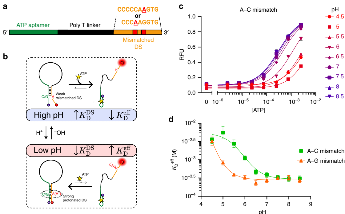
Fig. 3 Rational design of a high pH-specific ATP aptamer. a Preferential binding at neutral or alkaline pH is achieved by introducing an A-C or A-G mismatch into the DS sequence. b A simplified model for selective binding at higher pH. Mismatch protonation at acidic pH strengthens DS hybridization, decreasing the aptamer's effective affinity. A complete three-state model of the binding mechanism is given in Supplementary Fig. 5. c ATP binding curves for the A-C mismatch construct show increasing binding affinity at more alkaline pH. d Both A-C and A-G mismatches can be inserted to achieve stronger binding at neutral or alkaline pH than at acidic pH. Data points and error bars in c show the means and standard deviations of n = 3 independent experiments. Data points and error bars in d show the best fit values and standard deviations extracted from Langmuir isotherm fits to binding curve data from n = 3 independent experiments (data given in Supplementary Fig. 6) using nonlinear least squares fitting. Source data are provided as a Source Data file.
