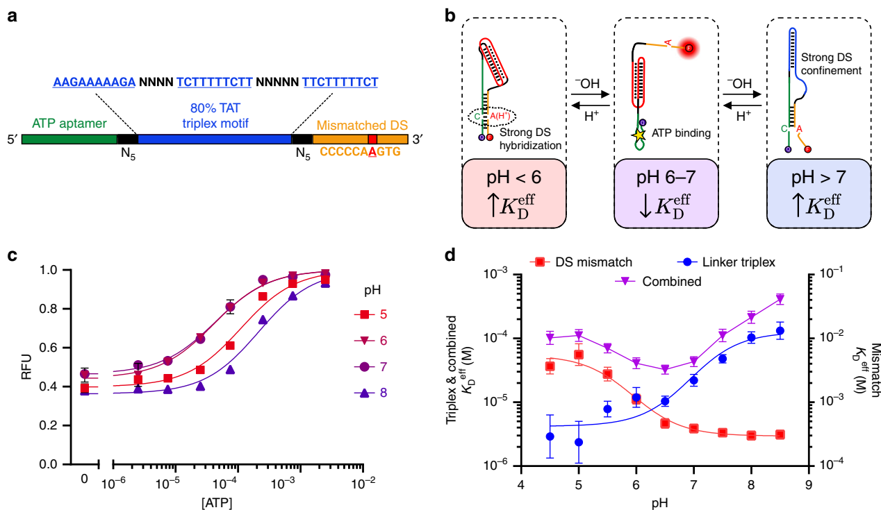
Fig. 4 PSD design for selective binding over a narrow pH window. a We designed a construct that incorporated both an intramolecular triplex in the linker domain and an A-C mismatch in the displacement strand. b Complex pH dependence is achieved through a three-state system, where binding is inhibited by strong DS hybridization at low pH or strong DS confinement at high pH, with a small window between these extremes where binding affinity is high. c ATP binding curves for the combined construct show the highest affinity at pH 6–7, with lower affinity at both high and low pH. d The pH dependence of affinity for this construct ( K_D^{\text{eff}} plotted on left axis) reflects contributions from both the binding inhibition of the linker modification-based TAT80 construct at high pH (left axis) and the binding inhibition of the DS modification-based A-C mismatch construct at low pH (right axis). Data points and error bars in c show the means and standard deviations of n = 3 independent experiments. Data points and error bars in d show the best fit values and standard deviations extracted from Langmuir isotherm fits to binding curve data from n = 3 independent experiments (data given in Supplementary Fig. 7) using nonlinear least squares fitting. Source data are provided as a Source Data file.
