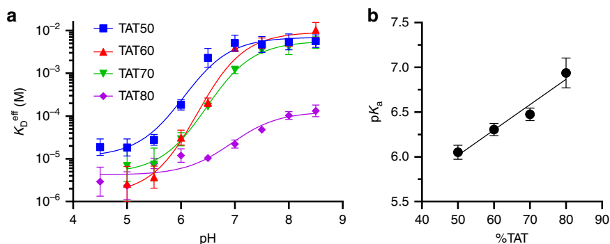
Fig. 2 pH response tuning through triplex base composition. a Constructs with varying TAT triplet compositions produce a range of pH dependencies, achieving selective binding at low pH but with varying magnitude of response and pH transition midpoint ( pK_a ). b Increasing the TAT content of the triplex motif predictably shifts the pK_a of the switch toward more neutral pH. Data points and error bars in a and b show the best fit values and standard deviations extracted from fits to binding curve data from n = 3 independent experiments (data given in Supplementary Fig. 4) using nonlinear least squares fitting. Source data are provided as a Source Data file.
