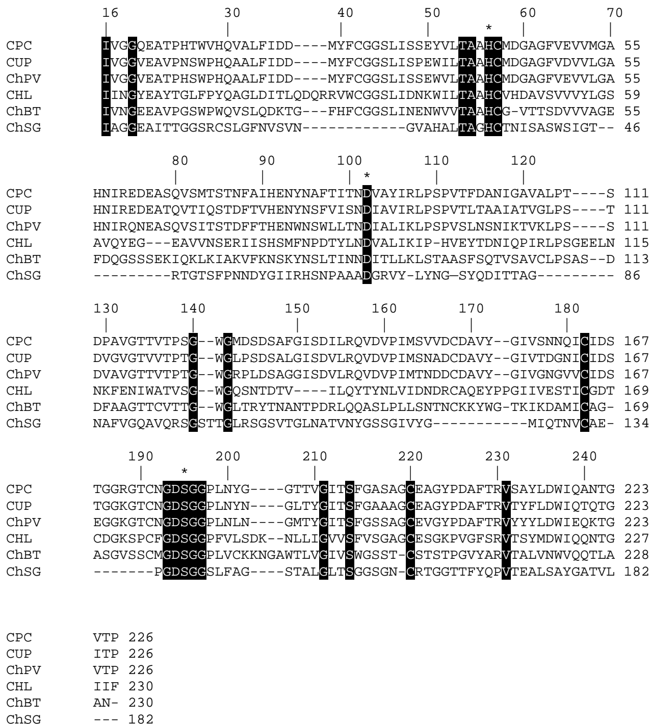
Figure 1 Alignment of amino acid sequences of collagenases and chymotrypsins. The completely conserved sites (13) are marked by black boxes. The catalytic triad (His, Asp, Ser) is denoted by stars above the sequences. Amino acid sequences are shown for: CPC, collagenase from P. camtschaticus (Q8VRI 1); CUP, collagenase from Uca pugilator (Q27824); ChPV, chymotrypsin II from Pen. vannamei (P36178); CHL, collagenase from Hypoderma lineatum (P08897); ChBT, chymotrypsin A from B. taurus (P00788); and ChSG, chymotrypsin-like protease from Streptomyces griseus (P00776). Swiss-Prot database accession numbers are given in parentheses. The numbers above the sequences follow the established chymotrypsinogen numbering system.
