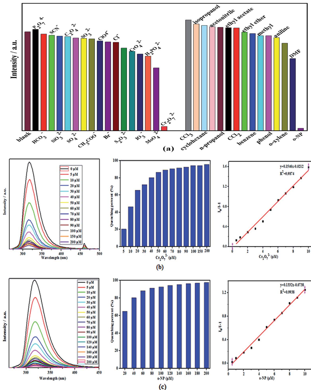
Fig. 5 (a) Luminous intensity of complex 1 (2 mL, prepared solution) in aqueous solutions with different \text{Cr} anions and organic small molecules (0.001 M). (b) Concentration-dependent luminescence quenching of complex 1 suspension in water by \text{Cr}_2\text{O}_7^{2-} (excited at 240 nm), percentage of luminescence quenching, Stern–Volmer plot of complex 1 suspension quenched by \text{Cr}_2\text{O}_7^{2-} . (c) Concentration-dependent luminescence quenching of complex 1 suspension in water by o -NP (excited at 240 nm), percentage of luminescence quenching, Stern–Volmer plot of complex 1 suspension quenched by o -NP.
