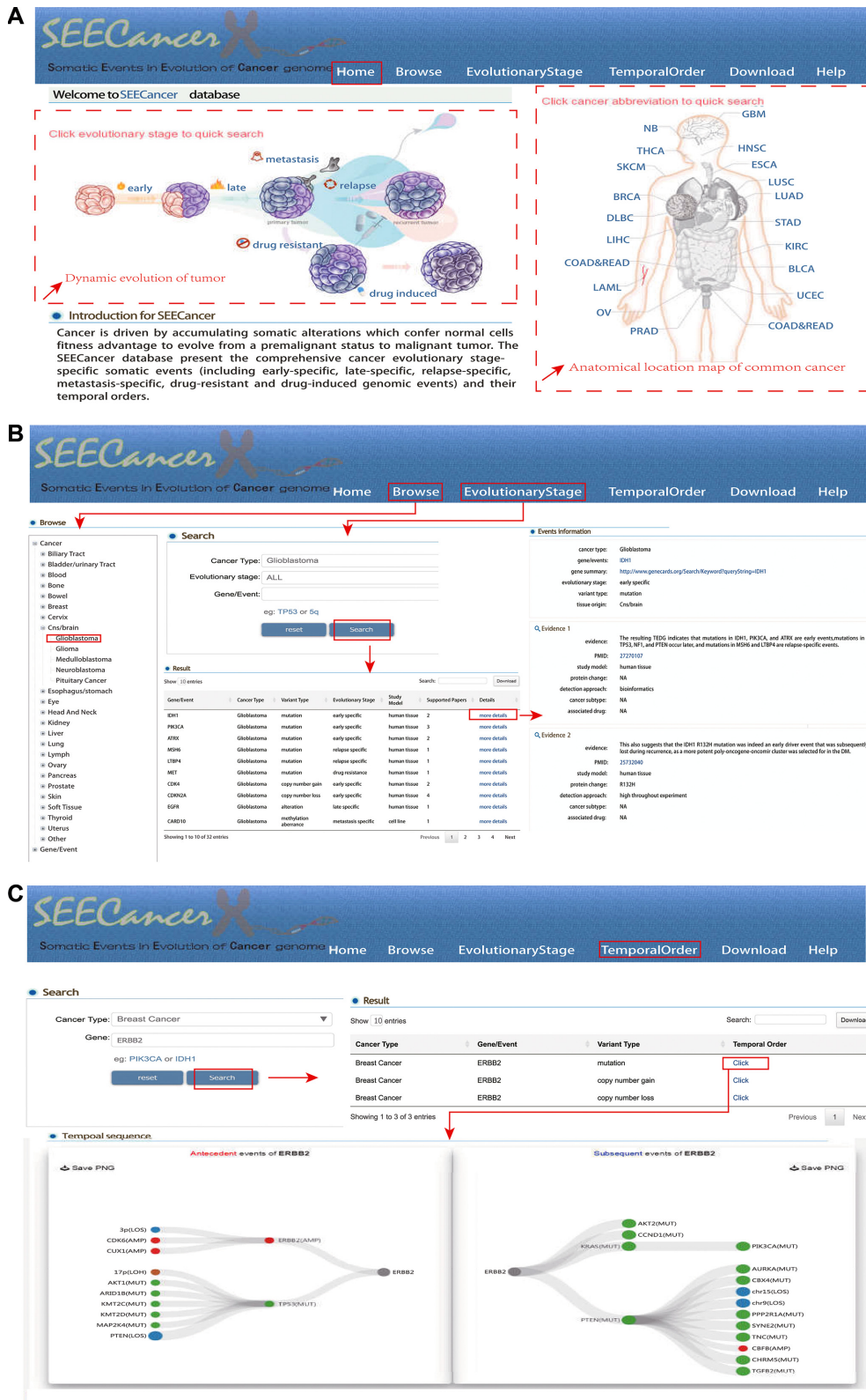
Figure 3. A schematic workflow of SEECancer. (A) The web images in the home page allow to quick research for evolutionary stage-specific events. (B) The 'Browse' and 'EvolutionaryStage' pages allow the users to browse and search evolutionary stage-specific events. (C) The 'TemporalOrder' page allows to search the antecedent events and subsequent events of queried alteration.
