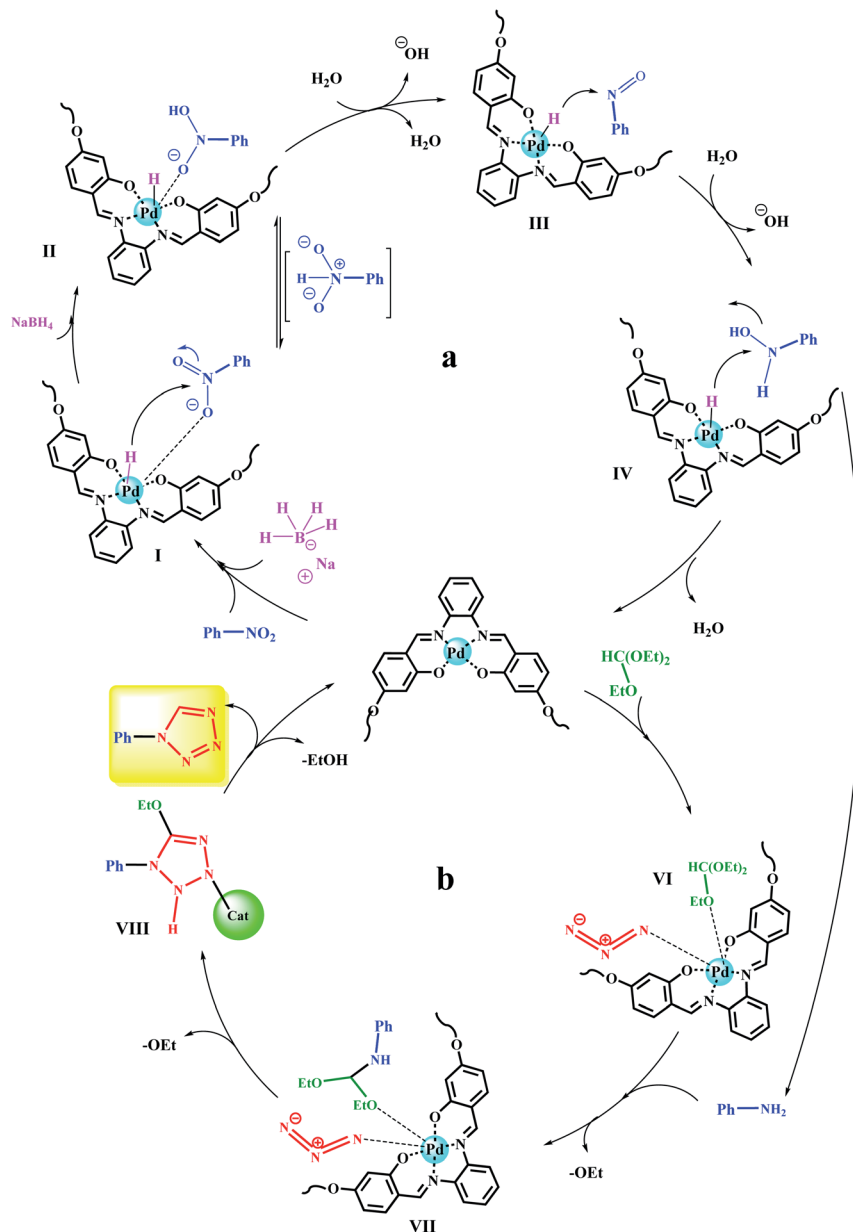
Scheme 7 Plausible reaction mechanisms for (a) reduction of nitroarenes and (b) their subsequent transformation to 1-substituted-1H-1,2,3,4-tetrazoles catalyzed by \text{Fe}_3\text{O}_4@ \text{SiO}_2@ \text{polysalophen-Pd(II)} .
