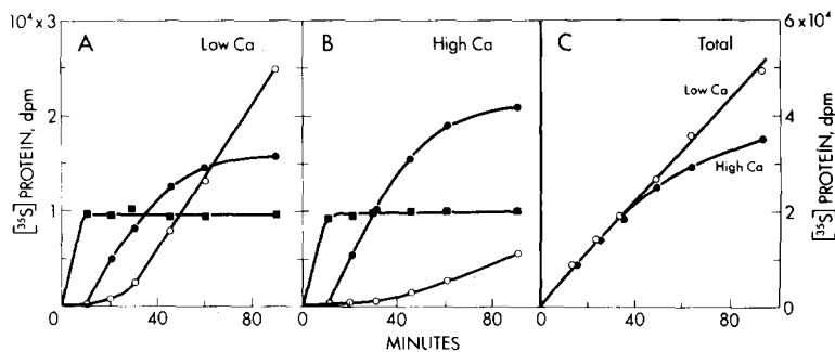
FIGURE 1 Continuous labeling study of the biosynthesis of radioactive parathormone and proparathormone and the secretion of the latter by porcine parathyroid cells. The cells were incubated in medium containing 25 \mu Ci/ml [ 35 S]methionine at either 0.5 (A) or 3.0 mM Ca (B). Samples of the incubation mixture were taken at the indicated times and the cells and medium were analyzed for hormonal protein as indicated under Materials and Methods. Total parathormone and proparathormone in the cells and medium at 0.5 and 3.0 mM Ca are portrayed in C. For A and B: \blacksquare — \blacksquare , proparathormone; \bullet — \bullet , cellular parathormone; \circ — \circ , secreted parathormone. For C: \bullet — \bullet , 3.0 mM Ca; \circ — \circ , 0.5 mM Ca.
