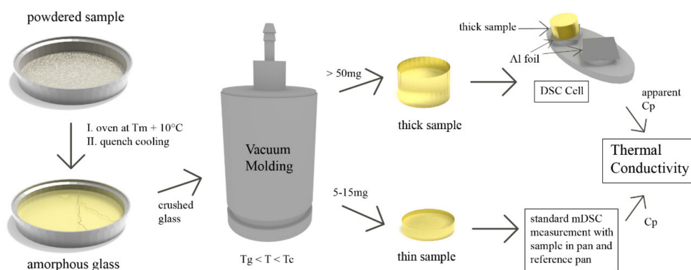
Figure 1. Sample preparation process and measurement schematic for the small molecule amorphous specimen.
