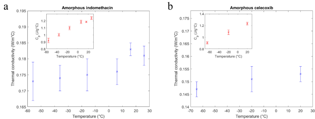
Figure 3. Thermal conductivity of indomethacin (a) and celecoxib (b). The insets show the specific heat capacity at the same measurement temperatures for the compounds, respectively.
