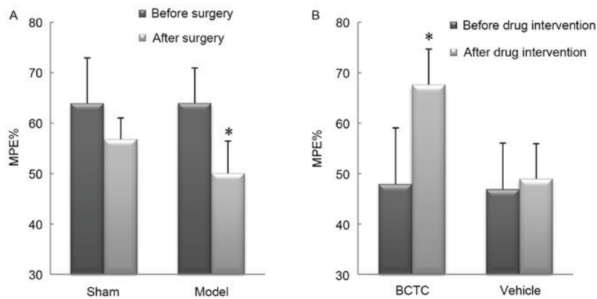
Figure 3. Tail flick latency in tail-flick test. (A) Bar chart of MPE% distributions in rats of sham and model groups before and after respective surgery. * P < 0.05 vs. MPE% before surgery. (B) Bar chart of MPE% distributions in BCTC and vehicle group 1 h before and after respective drug intervention. * P < 0.05 vs. MPE% before drug intervention. Data were presented as mean \pm standard deviation. Tail flick latency was presented as percentage of MPE. MPE, maximal possible effect.
