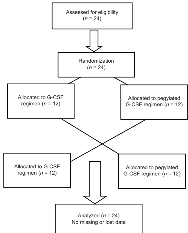
Figure 1: Consort diagram
