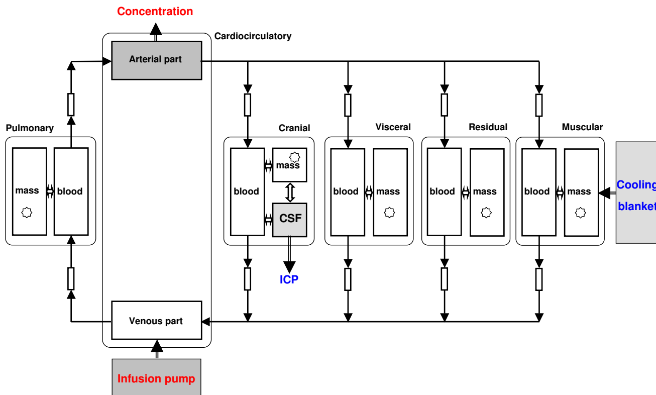
Figure 1 Structure of integrative model. Elevated ICP is reduced by therapeutic cooling [11]. Brain temperature, represented by CSF temperature, is reduced owing to therapeutic cooling. Propofol is administered into venous part of cardiocirculatory segment to achieve the minimum blood propofol concentration needed to inhibit thermoregulatory responses.
