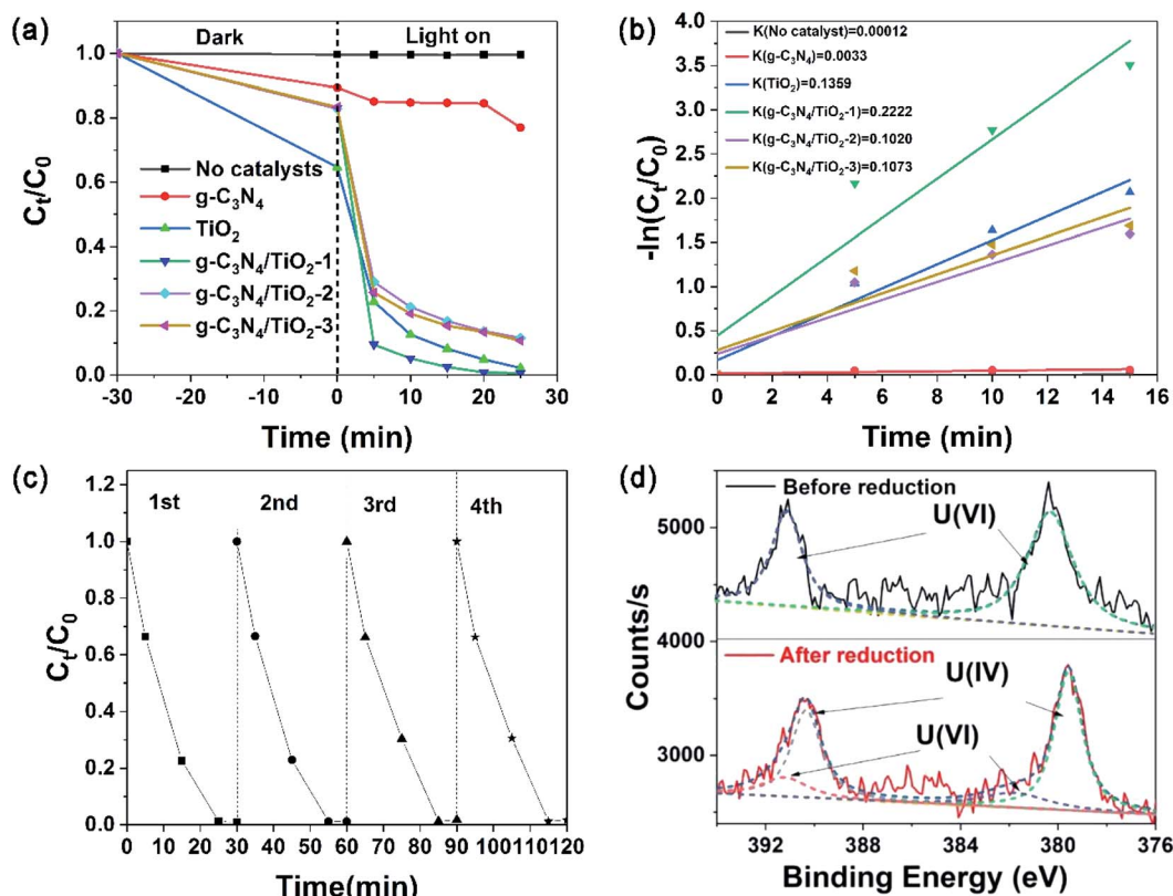
Fig. 4 (a) The variation of \text{U}(\text{vi}) during the reaction; (b) the rate constant ( k ) of \text{U}(\text{vi}) reduction; (c) cycling runs in the photocatalytic reduction of \text{U}(\text{vi}) ; (d) XPS spectrum of \text{U} 4f for the \text{U} element on the surface of g\text{-C}_3\text{N}_4/\text{TiO}_2 before (top) and after (bottom) reduction process.
