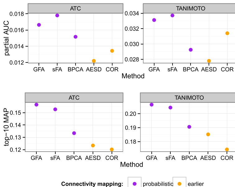
Figure 2 Probabilistic connectivity mapping outperforms earlier alternatives in retrieving similar drugs. The retrieval performance is indicated with two goodness measures (top row: partial AUC, bottom row: top-10 MAP) and two ground truths (left: ATC codes, right: Tanimoto similarity of the 2D fingerprints of the drugs). Probabilistic connectivity mapping (purple color) is performed with three models: Group Factor Analysis (GFA), sparse factor analysis (sFA), and Bayesian PCA (BPCA). These are compared to two earlier connectivity mapping methods (orange color): rank-based average enrichment-score distance (AESD) and the Pearson correlation over the differential expression profiles (COR).
