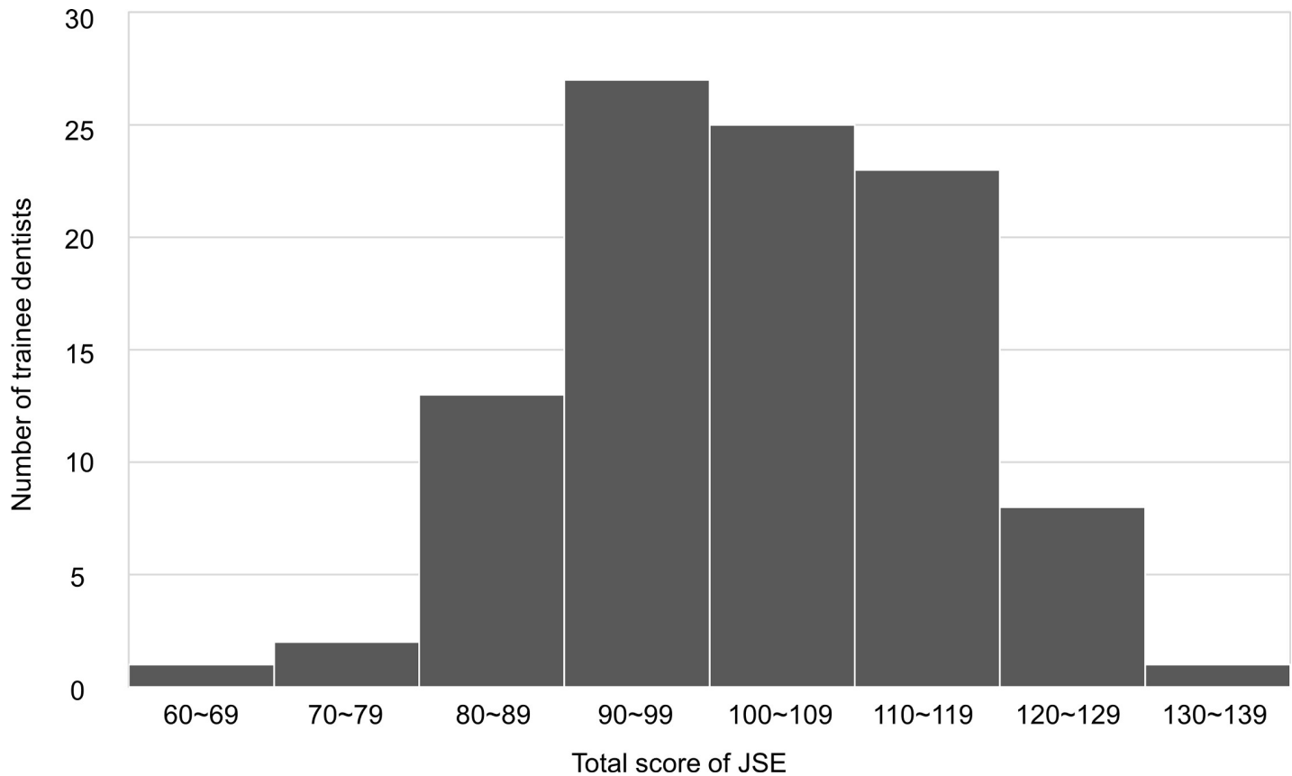
Fig 2. Distribution of total scores for the JSE.
