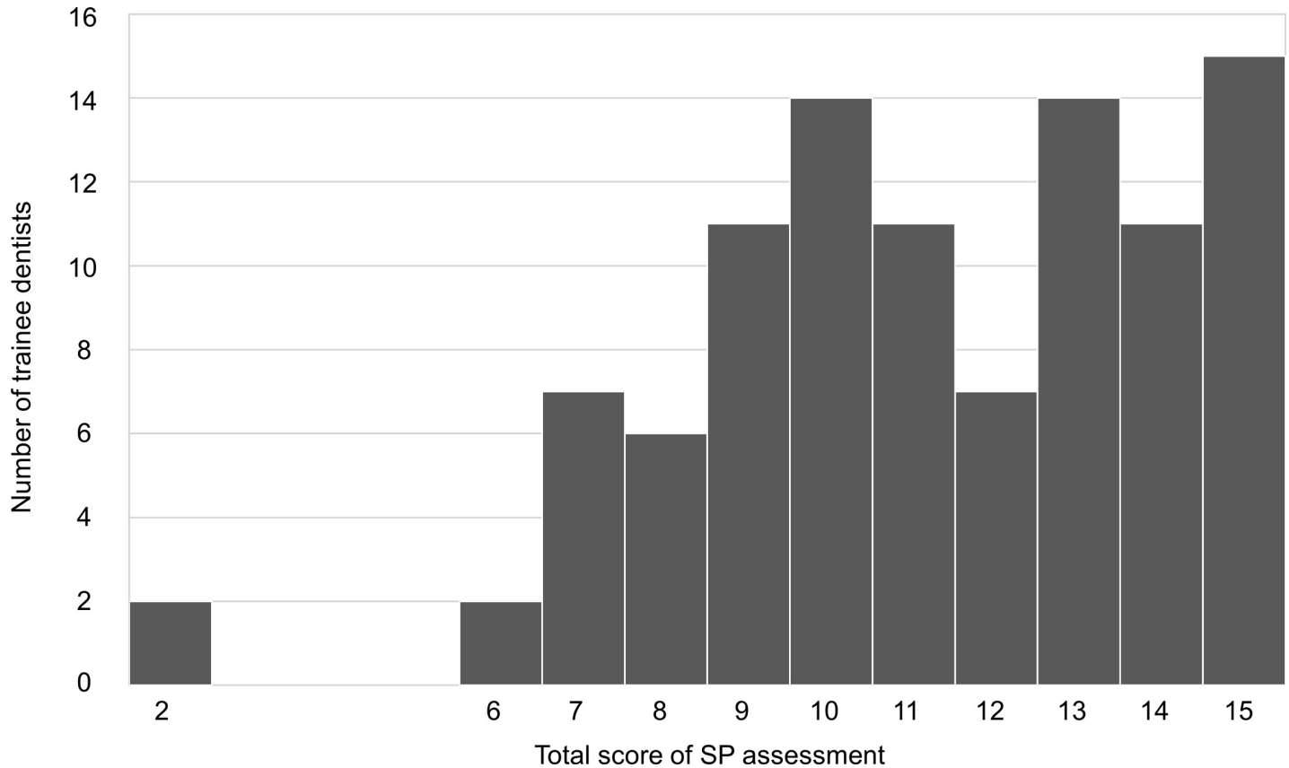
Fig 1. Distribution of total scores for SP assessment.
