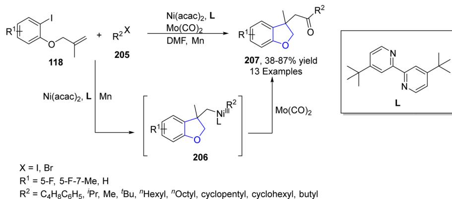
Scheme 45 Synthesis of 2,3-dihydrobenzofuran derivatives 207.
