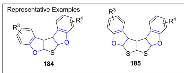
Scheme 38 Synthesis of furan-fused thienoacenes 182 – 185 .
