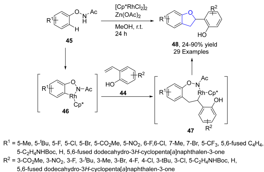
Scheme 5 Synthesis of 2,3-dihydrobenzofuran derivatives 48.
