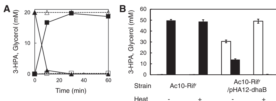
Figure 3 3-HPA production by simple biocatalyst. (A) Time course of 3-HPA production (squares) and glycerol consumption (triangles) from 20 mM glycerol in the reaction by Ac10-Rif r (dashed line, open marker) and Ac10-Rif r /pHA12-dhaB (solid line, filled marker). (B) Concentration of 3-HPA (light) and glycerol (black) in the reaction by Ac10-Rif r and Ac10-Rif r /pHA12-dhaB cells with (+) or without (-) heat treatment. Error bars represent standard deviation of the mean ( n = 3 ).
