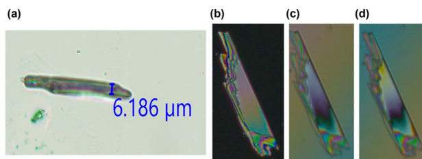
Fig. 5 (a) Thickness of a Li-4HP2 crystal and (b–d) a Li-4HP2 crystal observed under cross-polarized light, achieving complete extinction under a polarizing microscope.
