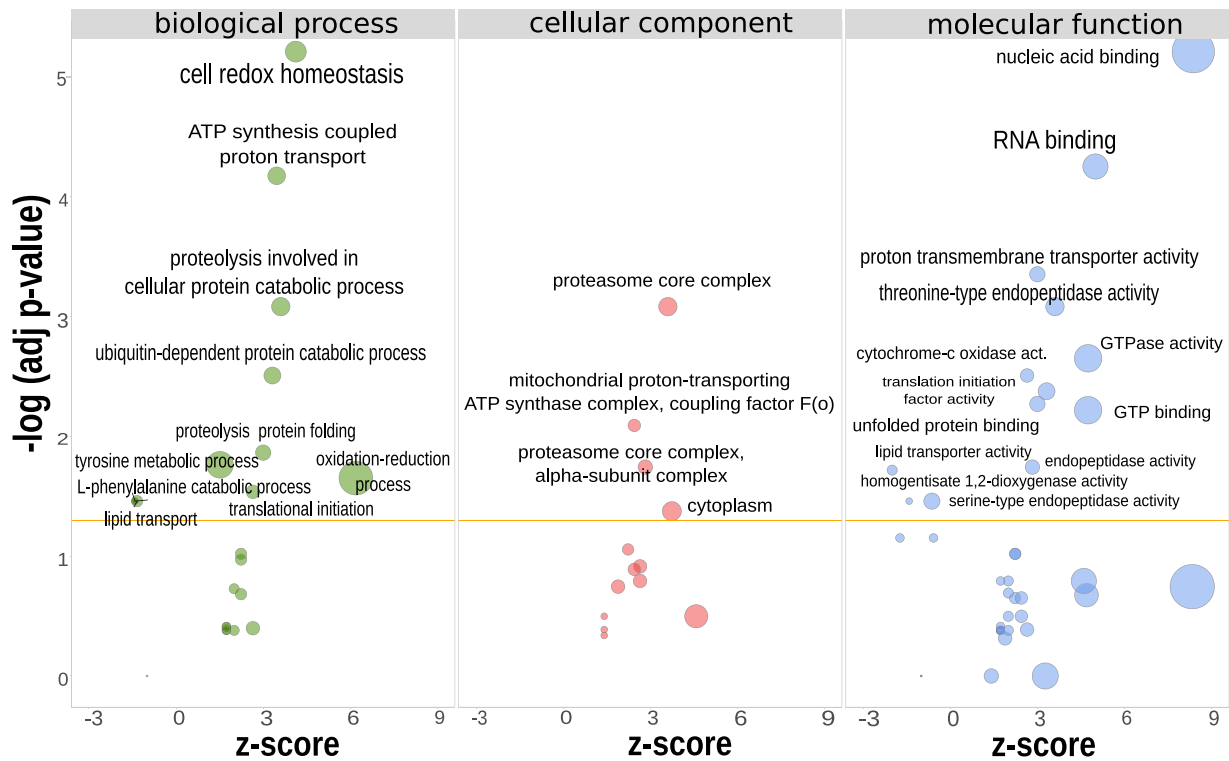
FIG. 6. —GO term enrichment analysis for DEGs in S. carcini interna and externa samples. The z-score is assigned to the x-axis. Negative values correspond to upregulation in the interna, whereas positive values correspond to upregulation in the externa. The y-axis shows the negative logarithm of the adjusted P -value (higher values are more likely to be significant). The area of the circles is proportional to the number of genes assigned to the term.
