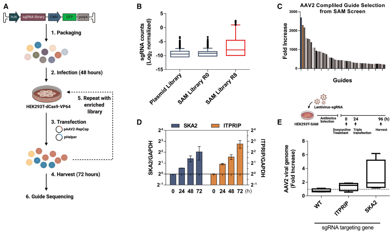
Figure 1. Parallel genome-wide screens identified candidate genes that increased HEK293 AAV manufacturing capacity
