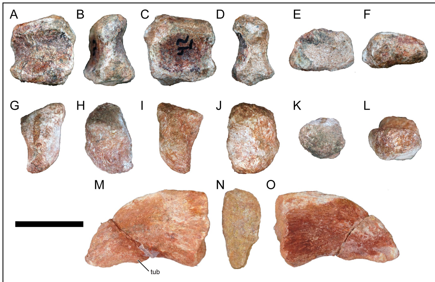
Fig 27. Pedal elements of Mnyamawamtuka moyowamkia . A–F, left pedal phalanx, and G–L, and M–O, left pedal unguals. A, G, M, dorsal; B, H, medial; C, I, plantar; D, J, O, lateral; E, K, proximal; F, L, distal views. Anterior t towards top of page in E, F, K, and L. Abbreviations: tub, tubercle. Scale bar equals 5 cm.
