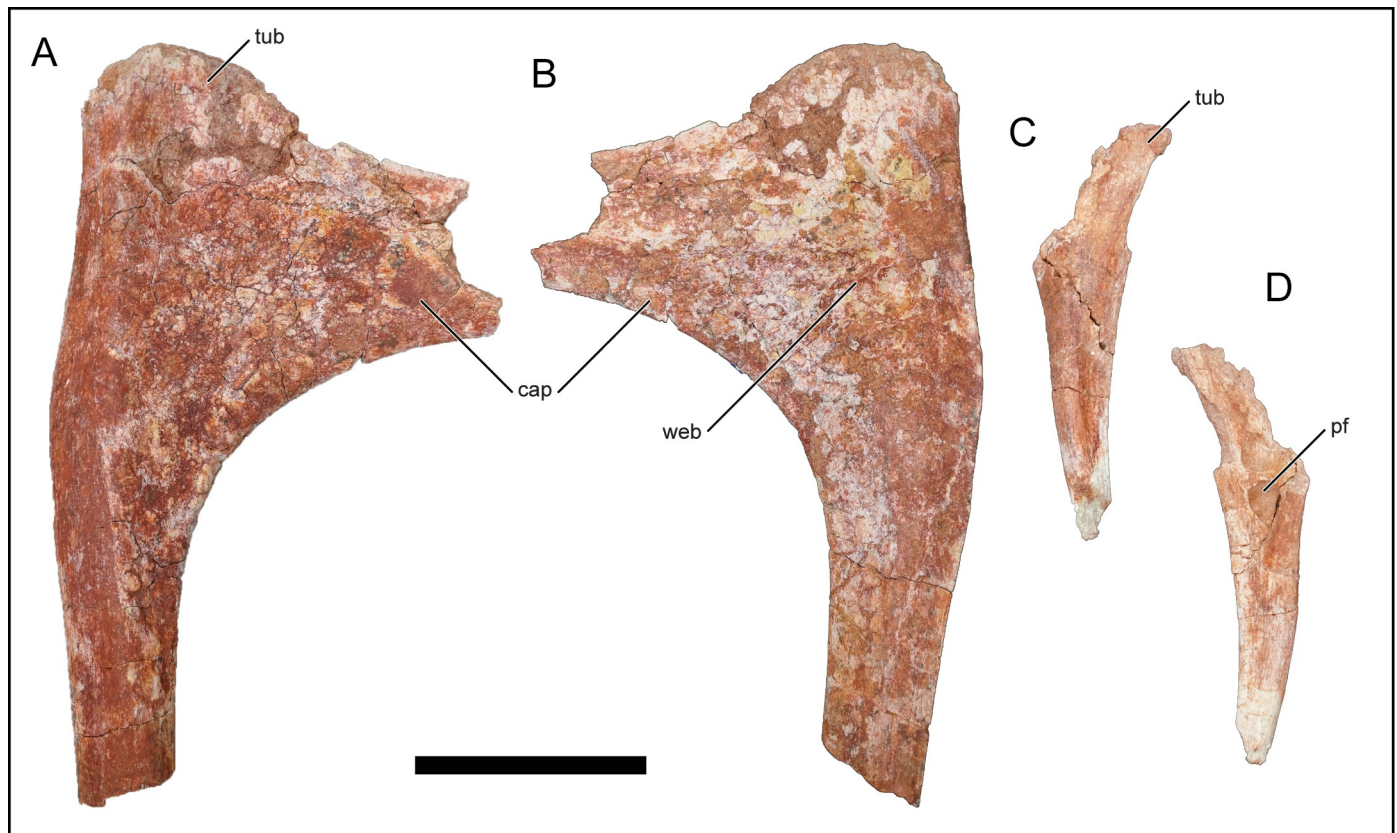
Fig 18. Dorsal ribs of Mnyamawamtuka moyowamkia . A–B, right anterior dorsal rib, and C–D, right posterior dorsal rib. A, C, anterior; and B, D, posterior views. Abbreviations: cap, capitulum; pf, pneumatic fossa; tub, tubercle; web, capitulotubercular webbing. Scale bar equals 10 cm.
