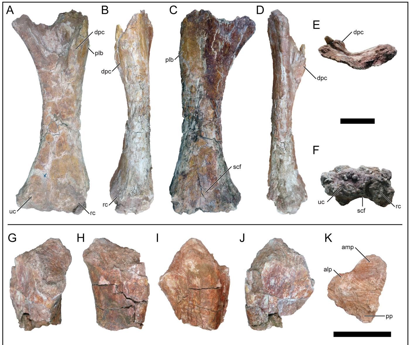
Fig 21. Forelimb elements of Mnyamawamtuka moyowamkia . A–F, left humerus, and G–K, partial left ulna. A, J, anterior; B, lateral; C, I, posterior; D, H, medial; E, proximal; F, distal; G, anteromedial; and K, cross section views. Anterior towards the top of the page in E, F, and K. Abbreviations: alp, anterolateral process; amp, anteromedial process; dpc, deltopectoral crest; plb, posterolateral bulge; pp, posterior process; rc, radial condyle; scf, supracondylar fossa; uc, ulnar condyle. Scale bars equals 10 cm.
