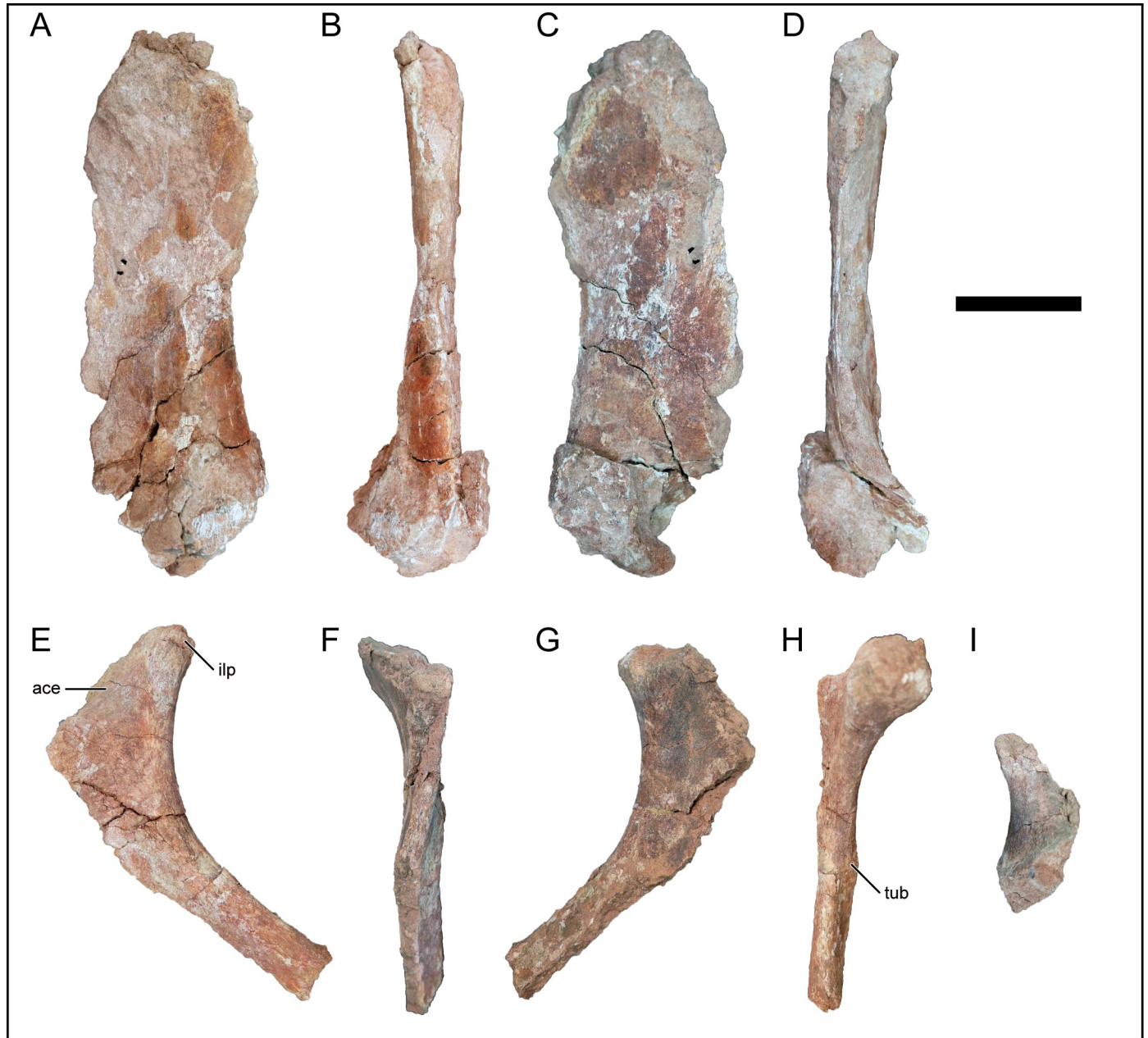
Fig 23. Pelvic elements of Mnyamawamtuka moyowamkia . A–D, right pubis, and E–I, right ischium. A, G, lateral/external; B, F, anterior; C, E, medial/internal; D, H, posterior; and I, proximal views. Anterior towards top in I. Abbreviations: ace, acetabulum contribution; ilp, iliac peduncle; tub, tubercle. Scale bar equals 10cm.
