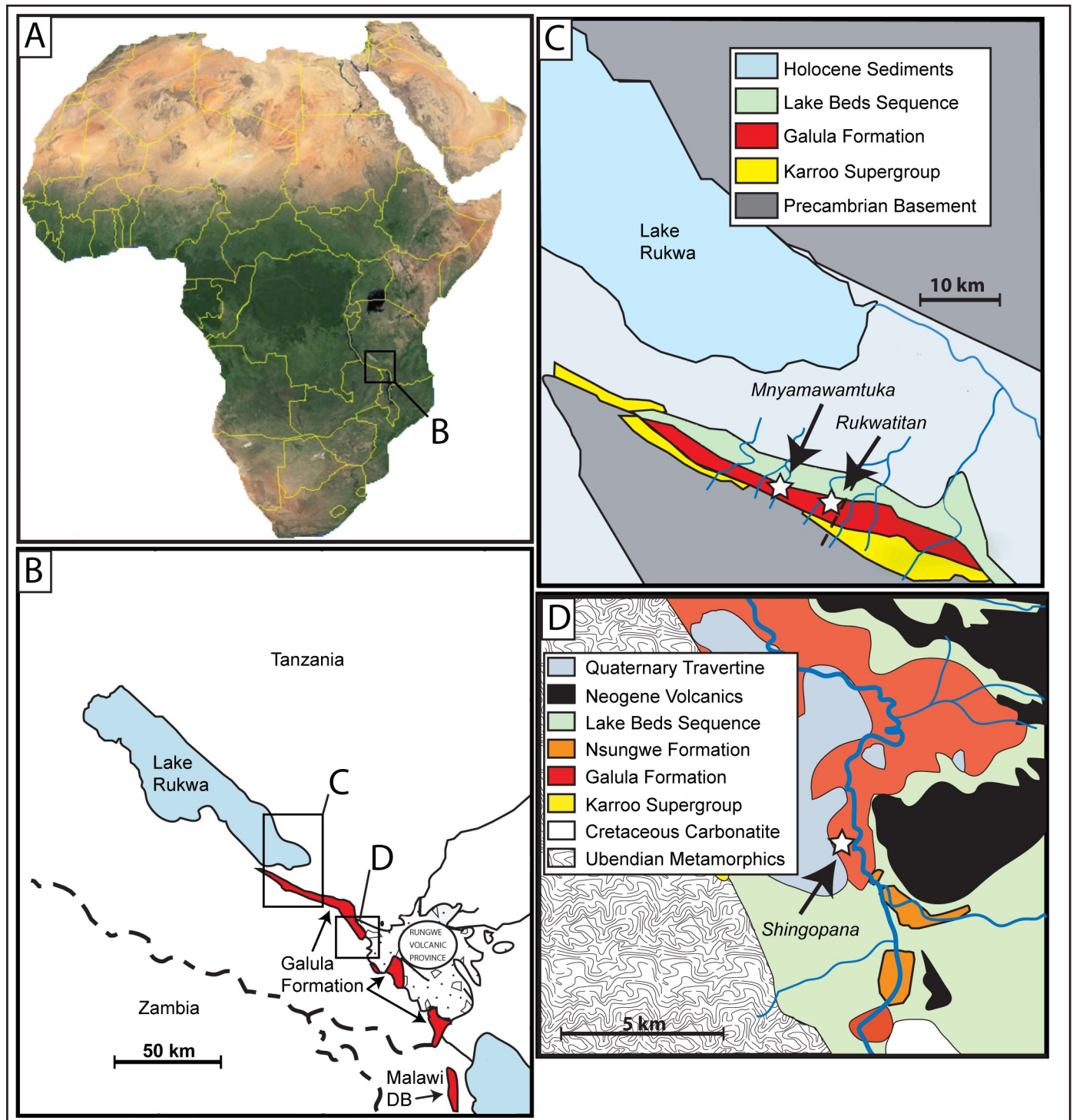
Fig 1. Map of research area. Map of Africa, A, with expanded regional map of the Rukwa Rift Basin of Tanzania, B, with the type localities of Mnyamawamtuka moyowamkia and Rukwatitan bispultus quarry near the Galula study area, C, and the Shingopana songwensis quarry near the Nsungwe study area, D. Malawi Dinosaur Beds (DB) marked in B to demonstrate the proximity of the deposits to the Galula Formation.
