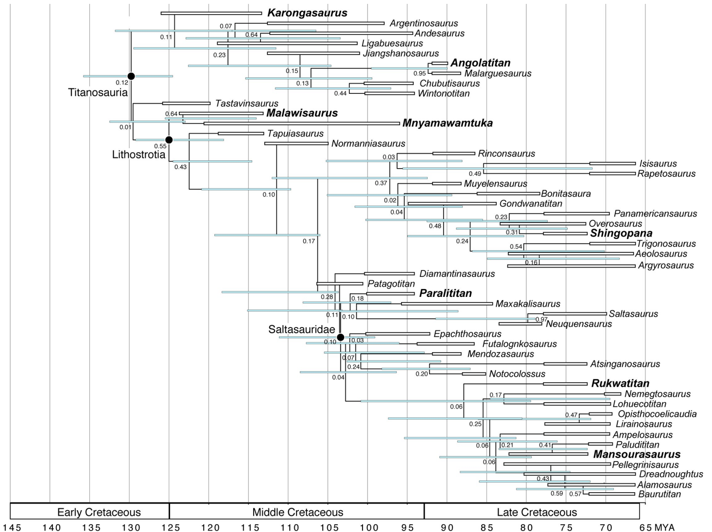
Fig 29. Results of tip-dating phylogenetic analysis. Maximum clade credibility tree for the variable-rates tip-dating Bayesian analysis. Numbers at the nodes represent posterior probabilities, blue bars at each node represent the 95% highest posterior density of each node age, and white bars at the tips represent the 95% highest posterior density of the sampled stratigraphic range of each terminal taxon. Abbreviations: MYA, millions of years ago.
