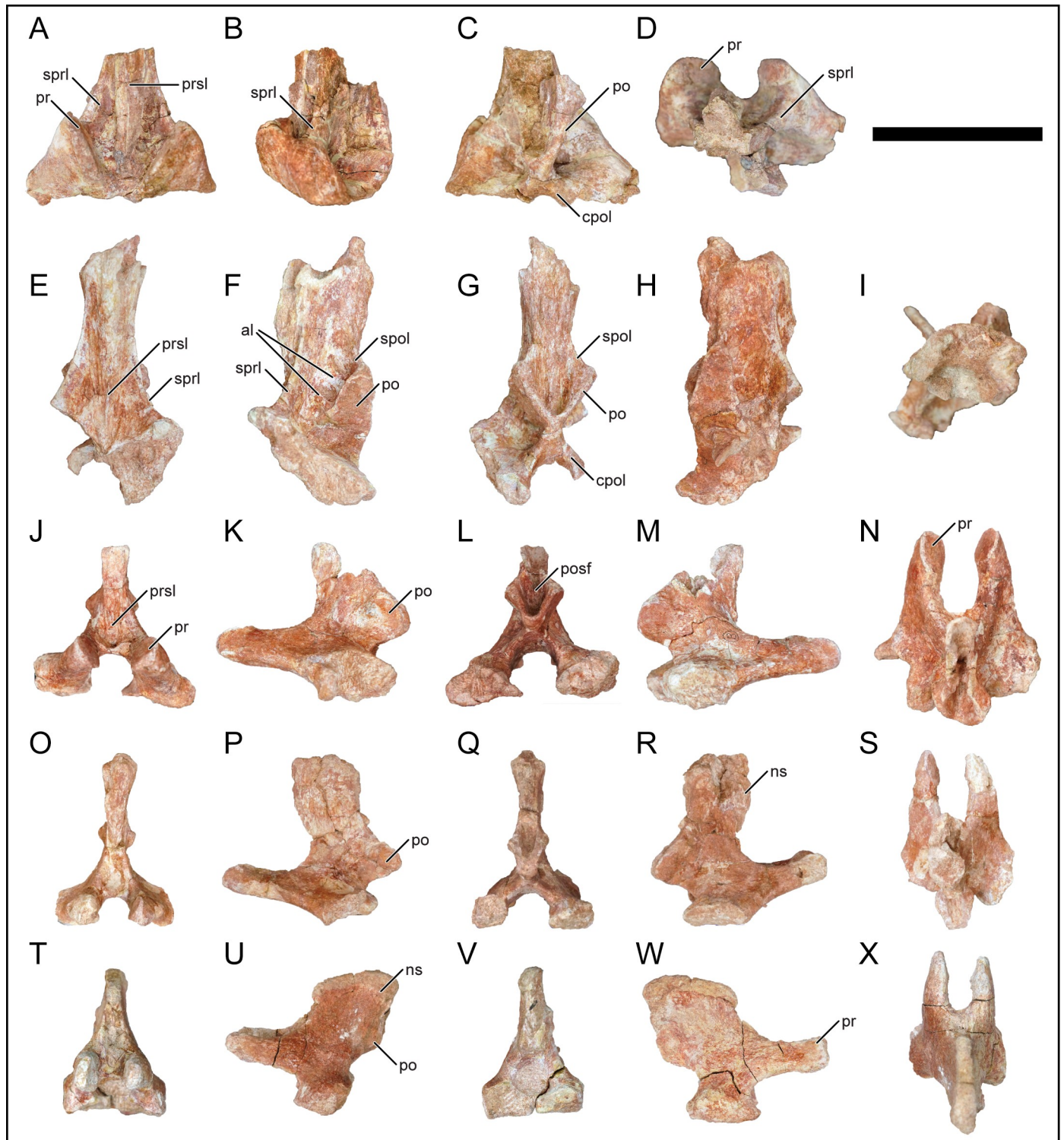
Fig 16. Caudal neural arches of Mnyamawamtuka moyowamkia . A–D, First caudal neural arch, E–I, anterior caudal neural arch, J–N and O–S, middle caudal neural arches, and T–X, posterior caudal neural arch. A, E, J, O, T, anterior; B, F, K, P, U, left lateral; C, G, L, Q, V, posterior; D, H, M, R, W, right lateral; and I, N, S, X dorsal views. Anterior towards the top in D, I, N, S, X. Abbreviations: al, accessory lamina; cpol, centropostzygapophyseal lamina; ns, neural spine; po, postzygapophysis; posf, postspinal fossa; pr, prezygapophysis; prsl, prespinal lamina; spol, spinopostzygapophyseal laminal; sprl, spinoprezygapophyseal lamina. Scale bar equals 10 cm.
