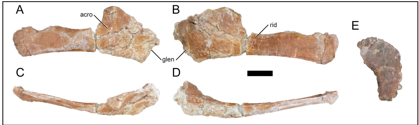
Fig 20. Pectoral elements of Mnyamawamtuka moyowamkia . A–D, right scapula, and E, right sternal plate. A, lateral; B, medial; C, dorsal; D, ventral; and E, external/ventral views. Abbreviations: acro, acromion; ant, anterior; art, articular facet for coracoid; glen, glenoid fossa; lat, lateral; med, medial; pos, posterior; rid, dorsomedial ridge of the scapular blade. Scale bar equals 10 cm.
