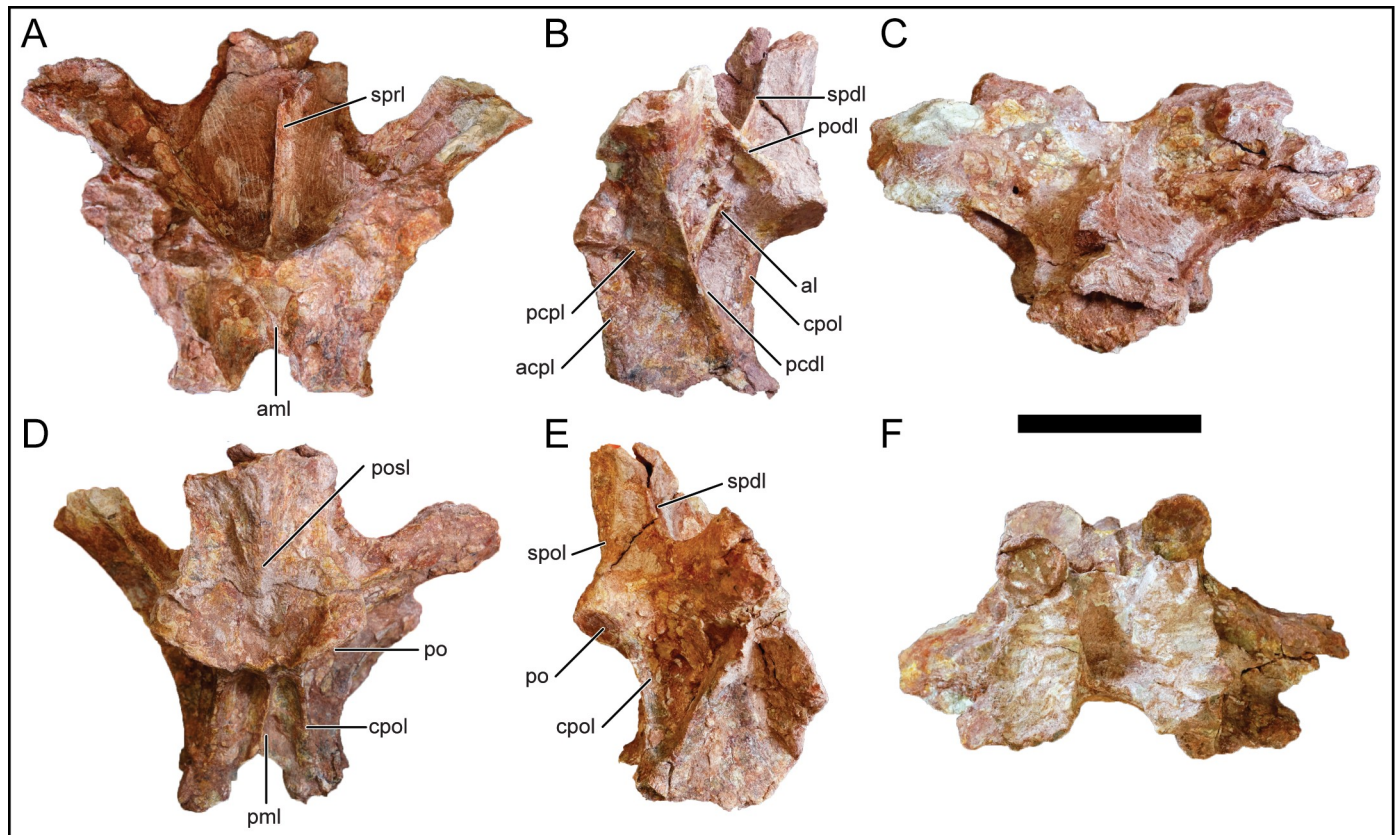
Fig 11. Posterior dorsal neural arch, D7, of Mnyamawamtuka moyowamkia . A, anterior; B, left lateral; C, dorsal; D, posterior; E, right lateral; and F, ventral views. Anterior towards the top of the page in C and F. Abbreviations: acpl, anterior centroparapophyseal lamina; al, accessory lamina; aml, anterior medial lamina; pcpl, posterior centroparapophyseal lamina; pml, posterior medial lamina; po, postzygapophysis; podl, postzygodiapophyseal lamina; posl, postspinal lamina; spdl, spinodiapophyseal lamina; spol, spinopostzygapophyseal lamina; sprl, spinoprezygapophyseal lamina. Scale bar equals 10 cm.
