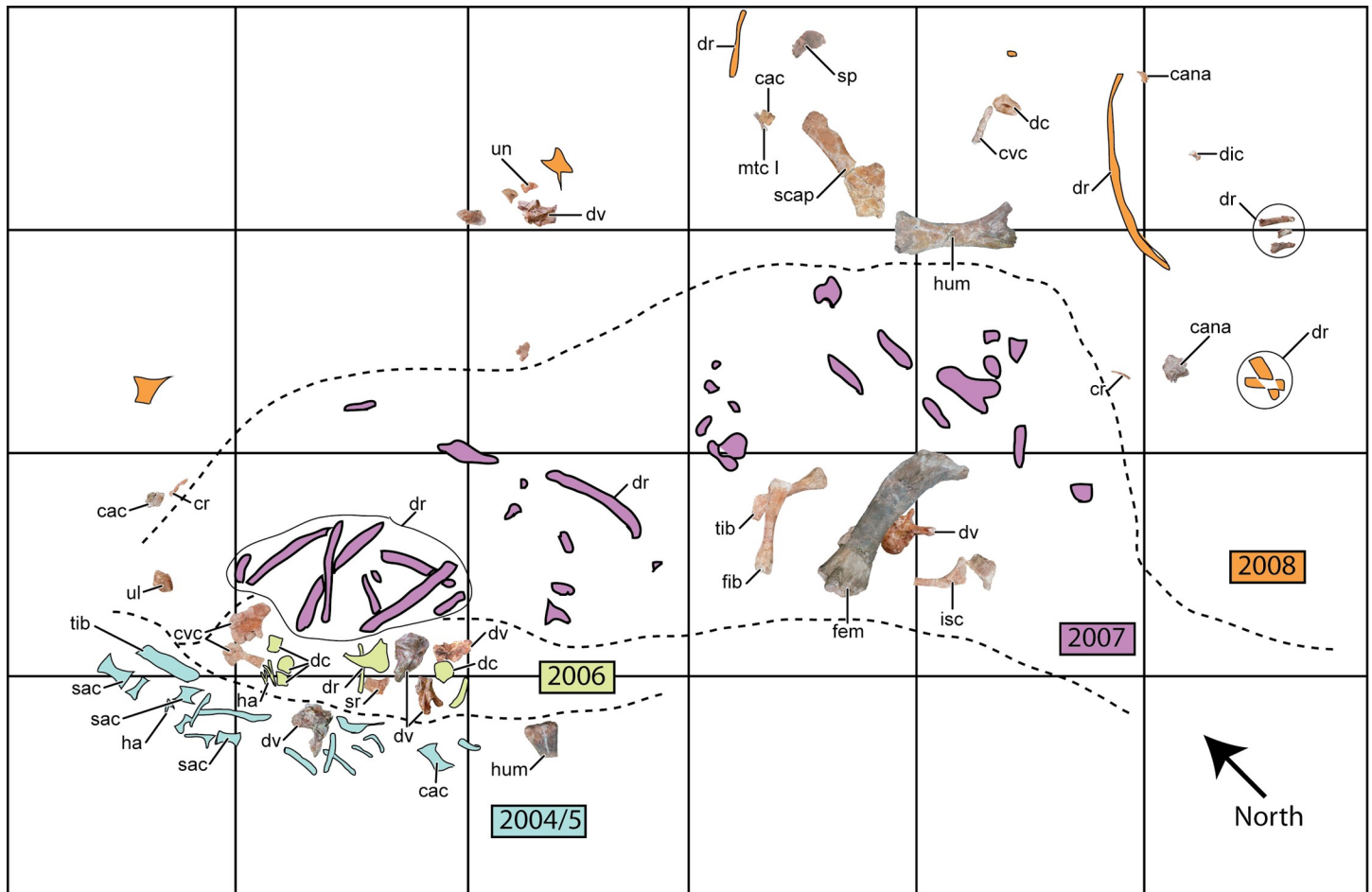
Fig 2. Quarry map. Quarry map of the Mtuka bonebed locality RRBP 2004–06. Recovered elements of M. moyowamkia are color-coded and separated by dashed lines according to the year they were collected. The quarry map is represented as a four-by-six-meter grid. Unmarked elements on the map are either fragments or unidentified. Abbreviations: cac, caudal vertebral centrum; cana, caudal vertebral neural arch; cr, cervical rib; cvc, cervical vertebral centrum; dc, dorsal vertebral centrum; dic, distal caudal vertebra; dr, dorsal rib; dv, dorsal vertebra; fem, femur; fib, fibula; ha, haemal arch; hum, humerus; isc, ischium; mtc I, metacarpal I; sac, sacral centrum; scap, scapula; sp, sternal plate; sr, sacral rib; tib, tibia; ul, ulna; un, ungual.
