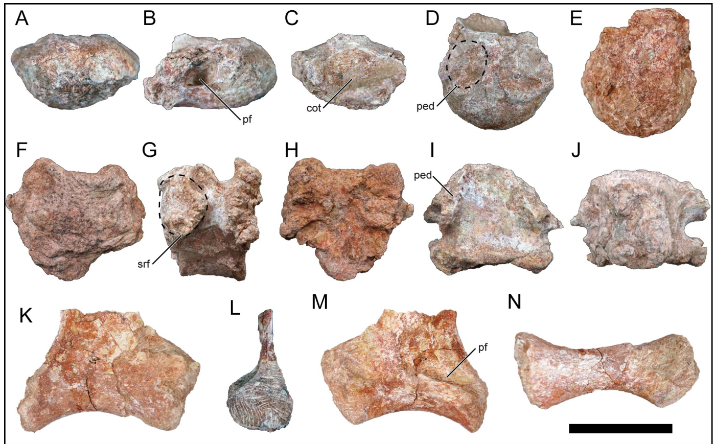
Fig 12. Sacral elements of Mnyamawamtuka moyowamkia . A–E, anterior sacral centrum; F–J, middle sacral centrum; and K–N, right sacral rib. A, F, M, anterior; B, G, left lateral; C, H, K, posterior; D, I, dorsal; E, J, N, ventral; and L, medial views. Anterior towards the top of the page in D, E, I, J, and N. Abbreviations: cot, cotyle; ped, site for fusion with pedicle; pf, pneumatic fossa; srf, sacral rib facet. Scale bar equals 10 cm.
