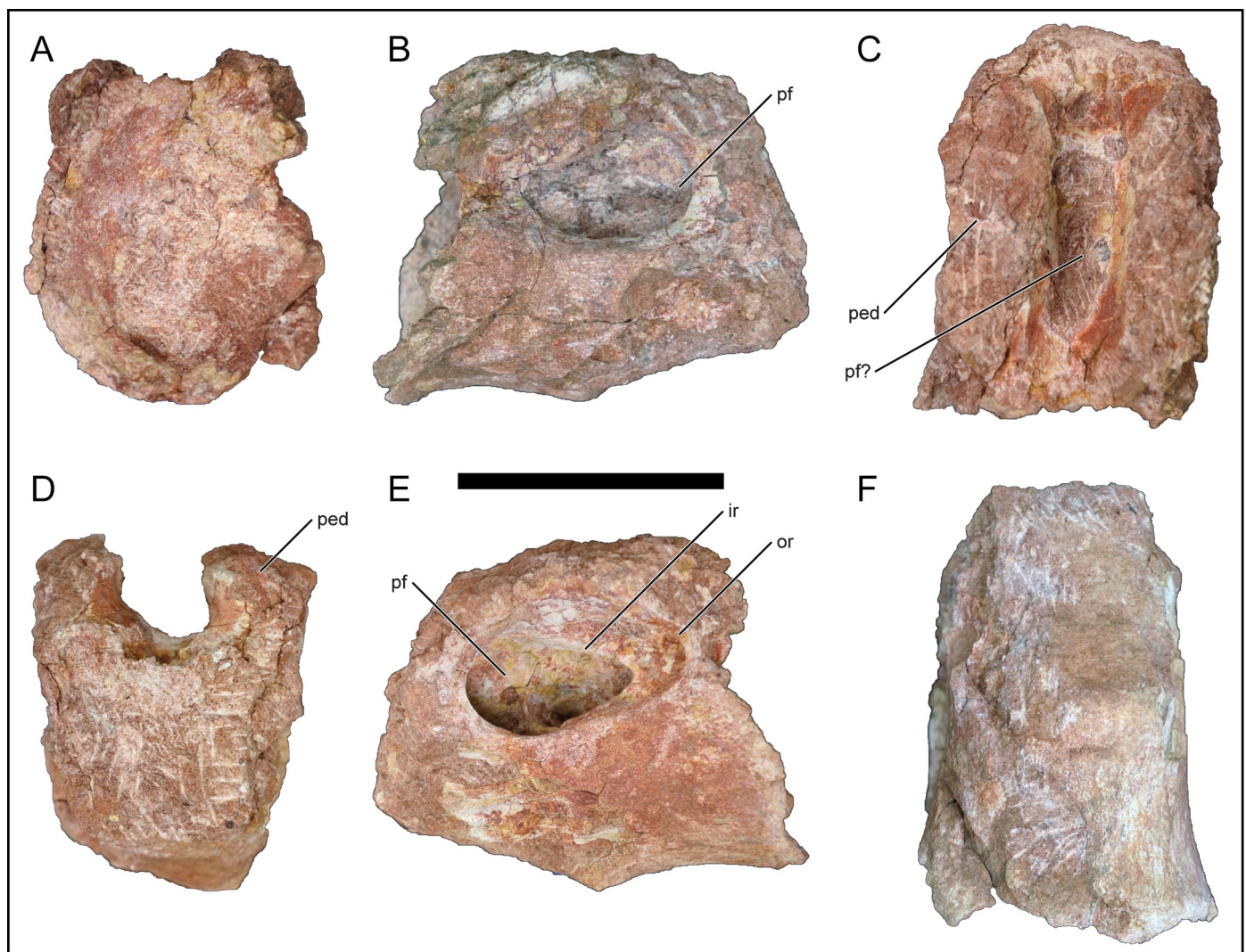
Fig 5. Example dorsal vertebra centrum of Mnyamawamtuka moyowamkia . A, anterior; B, right lateral; C, dorsal, D, posterior; E, left lateral; and F, ventral views; anterior to the top of page in C and F. Abbreviations: ir, inner rim of pleurocoel; or, outer rim of pleurocoel; ped, pedicle; pf, pneumatic fossa. Scale bar equals 10 cm.
