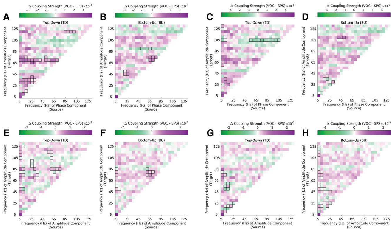
Figure 5. Phase-amplitude (PAC) and amplitude-amplitude (AAC) coupling strength in natural vocalizations (VOC) compared with synthetic envelope-preserved sounds (EPS) and synthetic spectrum-preserved sounds (SPS). A–D Difference in PAC strength between natural vocalizations and synthetic sounds. The difference between VOC and EPS stimuli ( A–B ) and between VOC and SPS ( C–D ) stimuli is depicted separately in the top-down and bottom-up direction. E–H Difference in AAC strength between natural vocalizations and synthetic sounds. The difference between VOC and EPS stimuli ( E–F ) and between VOC and SPS ( G–H ) stimuli is again depicted separately in the top-down and bottom-up direction. Significant differences are marked by black outlines ( p \leq 0.01 , cluster corrected). Results are depicted averaged across all channels, cross-regional pairs, and animals. See Extended Data Figure 5-1.
