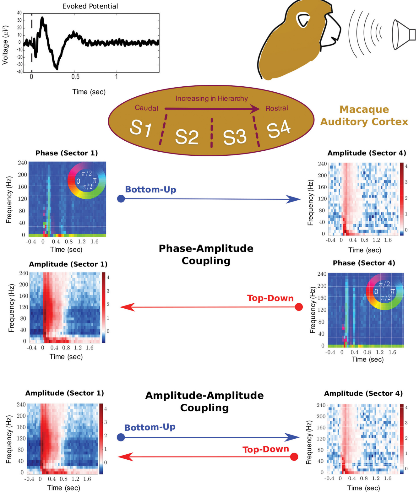
Figure 1. Coupling analysis overview: recordings were made from four \mu\text{ECoG} arrays spanning auditory cortex while monkeys listened to 1 of 20 natural VOCs, 20 synthetic EPSs, or 20 synthetic SPSs. Electrodes were partitioned into four sectors along the caudorostral axis (S1, A1/ML; S2, R/AL; S3, RTL; S4, RTp). We decomposed the signal into its time–frequency representation, and obtained amplitude and phase components for each sector. Plots of signal amplitude (in dB) are normalized to the baseline activity before stimulus onset. We investigated two types of coupling across sectors: amplitude–amplitude and phase–amplitude coupling. We computed both types of coupling in the bottom-up and top-down directions. Top-down coupling was defined as coupling in which
