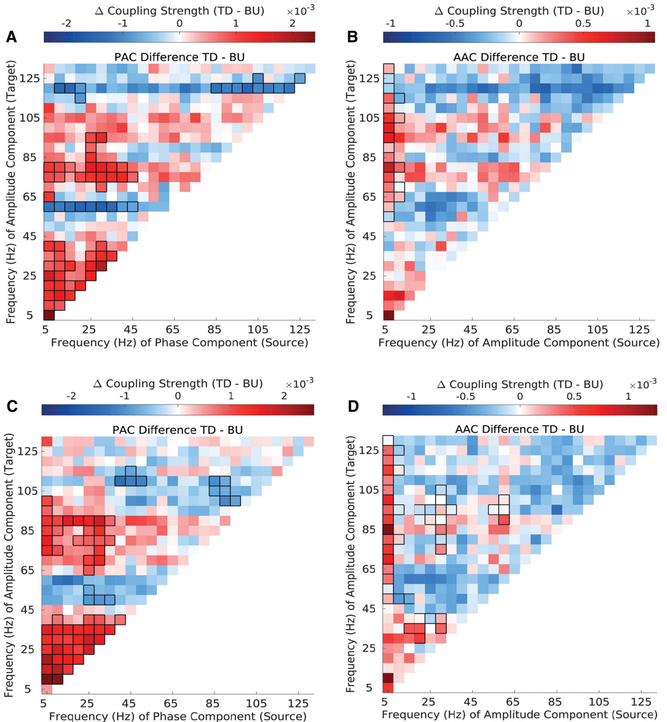
Figure 4. Top-down vs bottom-up phase–amplitude and amplitude–amplitude coupling in synthetic envelope-preserved stimuli (EPSs) and synthetic spectrum-preserved stimuli (SPSs) A , Difference in top-down and bottom-up PAC strength in EPS stimuli. B , Difference in top-down and bottom-up AAC strength in EPS stimuli. C , Difference in top-down and bottom-up PAC strength in SPS stimuli. D , Difference in top-down and bottom-up AAC strength in SPS stimuli. Significant differences are marked by black outlines ( p \leq 0.01 , cluster corrected). Results are depicted averaged across all channels, cross-regional pairs, and animals. See Extended Data Figure 4-1, Extended Data Figure 4-2, Extended Data Figure 4-3, Extended Data Figure 4-4, Extended Data Figure 4-5, and Extended Data Figure 4-6.
