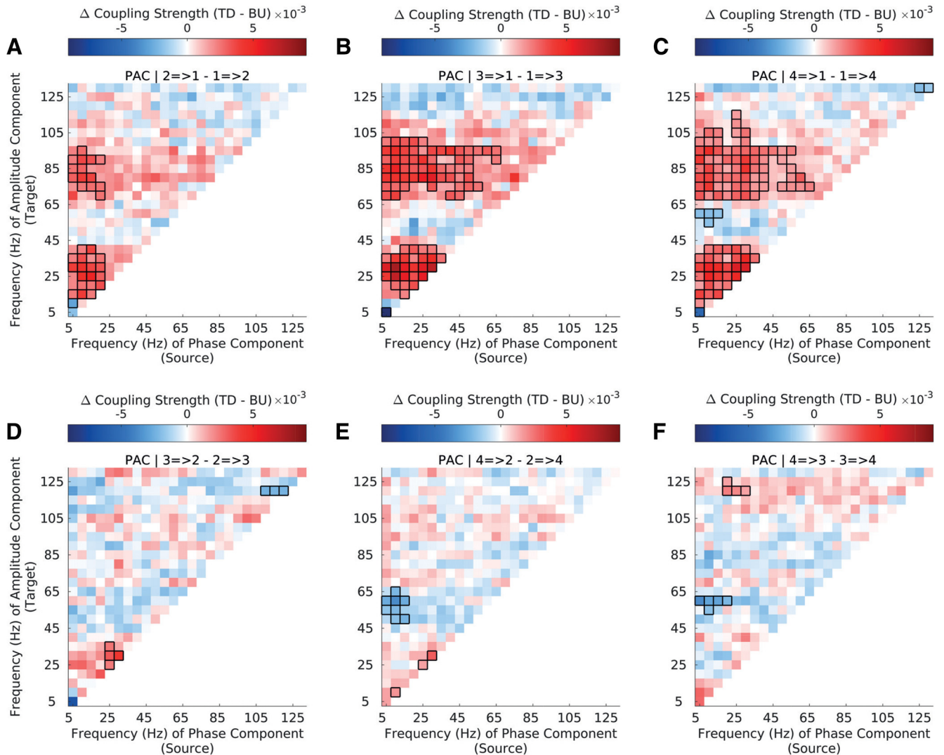
Figure 3. Top-down vs bottom-up PAC strength across the auditory hierarchy in natural stimuli. A–F , Difference in top-down and bottom-up PAC strength for CFC between sectors 1 (A1/ML) and 2 (R/AL; A ), sectors 1 (A1/ML) and 3 (RTL; B ), sectors 1 (A1/ML) and 4 (RTP; C ), sectors 2 and 3 ( D ), sectors 2 and 4 ( E ), and sectors 3 and 4 ( F ; for sector definitions, see Data preprocessing, in Materials and Methods). Interactions between sector 1 (A1/ML) and higher-order sectors show strong asymmetries in bottom-up and top-down coupling strength across the frequency spectrum; interactions among higher-order sectors (S2–S4) show less widespread asymmetries. Significant differences are marked by black outlines ( p \leq 0.01 , cluster corrected). Results are depicted averaged across all channels and animals. See Extended Data Figure 3-1.
