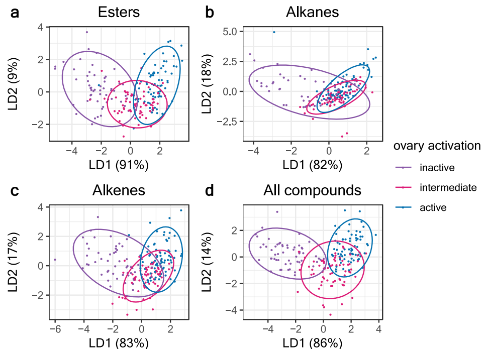
Figure 3. Linear discriminant analyses on Z-transformed relative peak areas of Dufour's gland extracts of workers with three ovarian activation categories as the grouping variable. Each point is the value from an individual bee. Panels (a–d) show the clustering generated by plotting the first two linear discriminant functions using esters, alkanes, alkenes, or all compounds.
