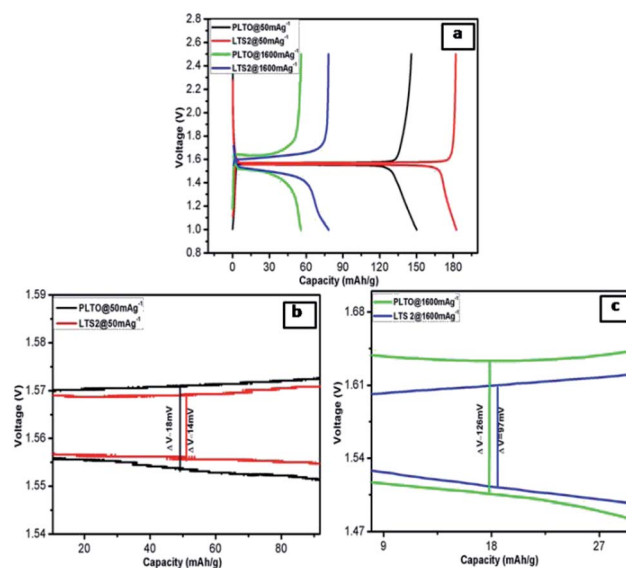
Fig. 10 (a) Comparison of the initial discharge-charge profiles of PLTO and LTS2 at 50 and 1600 \text{ mA g}^{-1} and (b) 50 \text{ mA g}^{-1} (c) 1600 \text{ mA g}^{-1} .
