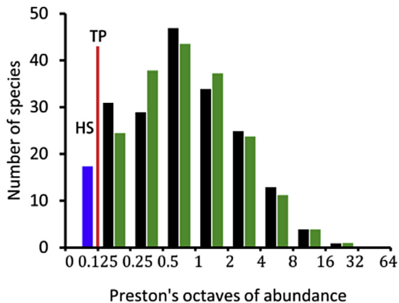
Fig. 7. A plot of truncated lognormal distribution of species abundances in Preston's octaves (abundance classes) following Pielou's (1975) method of fitting. The observed frequencies of species in octaves are shown in black bars, expected frequencies in green bars and the frequency of hidden species in the blue bar (HS). The red line marked with TP indicates the truncation point.
