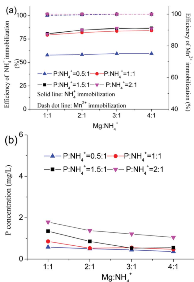
Fig. 4 Immobilization of contaminants (a), and the change in the P concentration (b) using PO agents.
