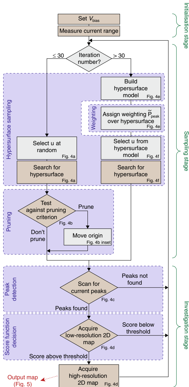
Fig. 3 Flow diagram of the algorithm. (See text and Fig. 4 for a full description.) Each step is annotated with the corresponding panel in Fig. 4. Steps that involve interaction with the device are shaded brown, and entirely computational steps are grey. In the ablation studies of Section “Ablation study”, the different modules that constitute the algorithm are studied in terms of their contribution to the algorithm’s performance; these modules are marked by the blue background regions. The steps belonging to the initialisation, sampling, and investigation steps are indicated on the right.
