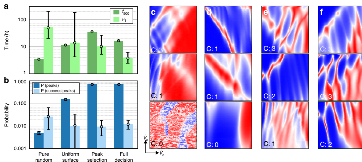
Fig. 6 Ablation study. a, b Bar charts and corresponding data points comparing \mu_t (light green), t_{500} (dark green), P(\text{peaks}) (dark blue) and P(\text{success}|\text{peaks}) (light blue) for the different algorithms considered. Error bars represent 80% (equal-tailed) credible intervals. Due to a measurement problem, 459 sampling iterations instead of 500 were considered for the Full decision algorithm. c-f High resolution current maps sampled by pure random, uniform surface, peak weighting, and full decision, respectively. In each panel, we indicate C, the number of human labellers that identified a map as displaying double quantum dot features. Current maps with identical values of C are displayed in the order in which they were sampled, from top to bottom. Current maps with C: 0 were randomly selected. Each panel uses an independent colour scale running from red (highest current measured) to blue (lowest current).
