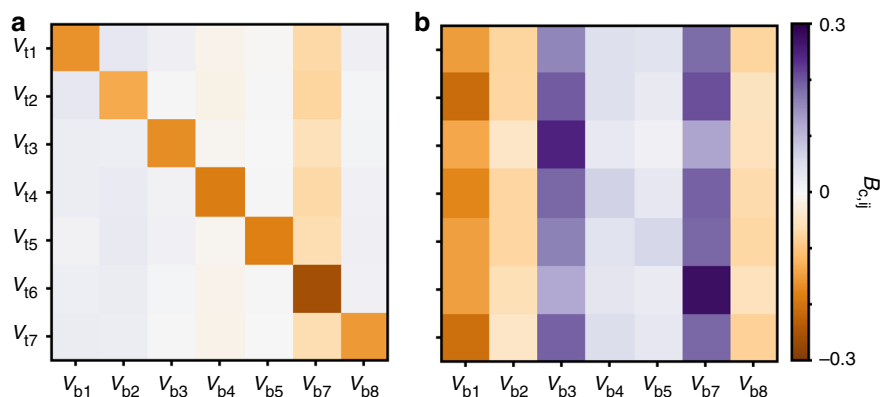
Fig. 7 Learning about device variability. B_c matrices obtained using point set registration. Indices are the gate voltage locations \mathbf{v}_b and \mathbf{v}_t . V_6 = 0 mV was fixed in Device 2 to prevent leakage currents. a Transformation between the hypersurface of Device 2 before and after a thermal cycle. b Transformation between the hypersurfaces of Device 1 and Device 2.
