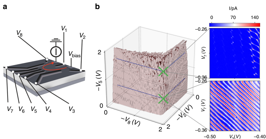
Fig. 1 Overview of device, and gate voltage space. a Schematic of a gate-defined double quantum dot device. b Left: Boundary hypersurface measured as a function of V_2 , V_5 , and V_8 , with fixed values of V_1 , V_3 , V_4 , V_6 , and V_7 . The current threshold considered to define this hypersurface is 20% of the maximum measured current. The gate voltage parameter space, restricted to 3D for illustration, contains small regions in which double and single quantum dot transport features can be found. These regions typically appear darker in this representation because they produce complex boundaries. Right: For particular gate voltage locations marked with green crosses, the current as a function of V_7 and V_3 is displayed. The top and bottom current maps display double and single quantum dot transport features, respectively.
