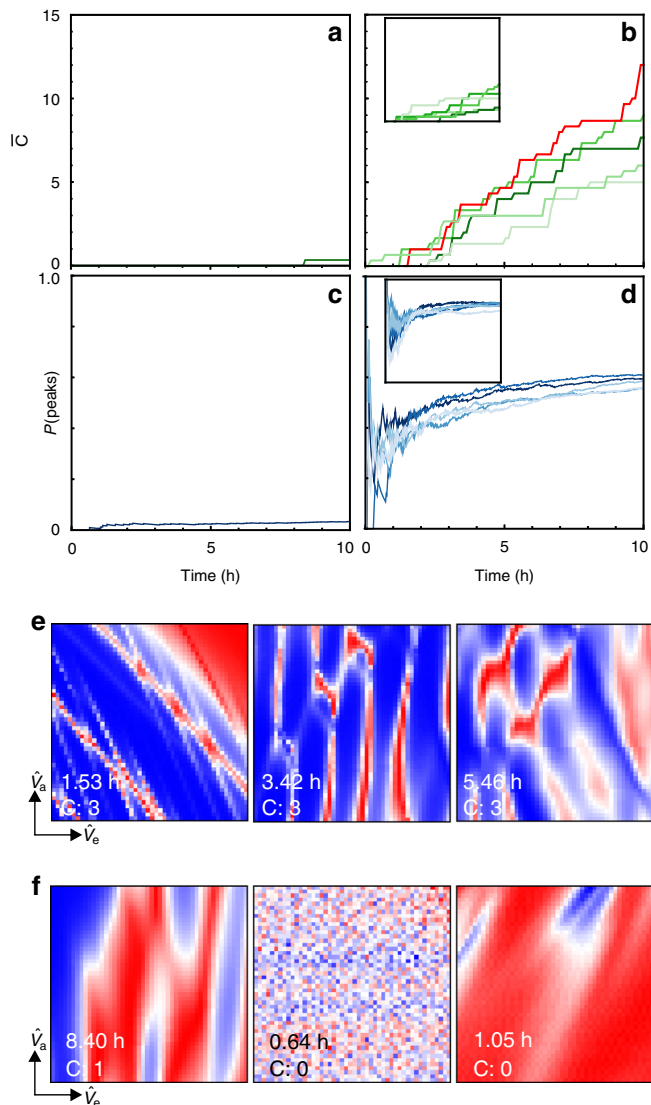
Fig. 5 Algorithm's performance. a–d Average number of current maps displaying double quantum dot features, \bar{C} , and P(\text{peaks}) as a function of laboratory time. Current maps are labelled by humans a posteriori, i.e., after the algorithm is stopped. a, c, b, d correspond to one run of Pure random and five runs of our algorithm, respectively. All algorithm runs displayed in main panels were performed in Device 2, while insets show runs of our algorithm in Device 1. e, f High resolution current maps measured in Device 2 by Pure random and one of our algorithm runs, respectively. We indicate the time the algorithm had been running for before they were acquired and the number of labellers, C , that identified them as displaying double quantum dot features. Current maps are ordered from left to right in decreasing order of C , and maps that have the same values of C are displayed in the order at which they were sampled. Each panel uses an independent colour scale running from red (highest current measured) to blue (lowest current).
