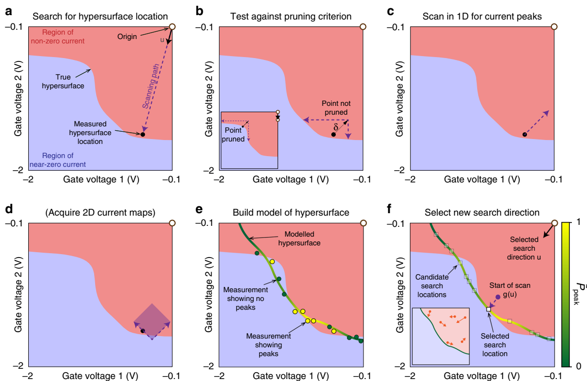
Fig. 4 Characterising the boundary hypersurface using machine learning. Each panel illustrates a step of the algorithm presented in Fig. 3. The gate voltage space, restricted to two dimensions for illustration, is divided into regions of near-zero (blue) and non-zero current (pink), separated by a boundary hypersurface. a Locating the hypersurface. The gate voltages are scanned along a ray (violet arrow) starting at the origin (white circle) and defined by direction \mathbf{u} . By monitoring the current, the intersection with the hypersurface is measured. b To determine whether a region should be pruned, the algorithm scans each gate voltage individually toward the bottom of its range from a location just inside the hypersurface as shown. If only one scan intersects the hypersurface (as in the inset), future exploration of that region is inhibited by displacing the origin as shown. c Based on a short 1D scan, the location is classified according to whether it shows current peaks indicating Coulomb blockade. d If peaks are found, a 2D scan (violet square) is performed in the plane of V_3 and V_7 , and is possibly repeated at higher resolution. e From the first thirty measurements (green and yellow circles), the algorithm builds a model of the hypersurface and assigns a probability \tilde{P}_{\text{peak}} that peaks will be found. f To refine the model, the algorithm generates a set of candidate search locations (squares), each weighted by its corresponding value of \tilde{P}_{\text{peak}} , and selects one at random. A new scan is then performed in the corresponding direction to generate a new measurement of the hypersurface location. Steps d-f are then repeated indefinitely. Inset: Scheme for numerically sampling the hypersurface using simulated Brownian motion. Each point represents a simulated particle moving inside the enclosed volume. The collisions between the particles and the modelled hypersurface generate a set of candidate search locations.
