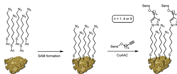
Scheme 2 Schematic representation of the npAu hybrid preparation; formation of an azide terminated SAM using 6-azidothioacetate followed by attachment of the different photosensitizers via CuAAC (“click reaction”).
