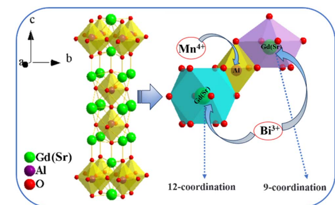
Fig. 1 Structure framework of SGAO compound and Gd(Sr)–O, Al–O polyhedrons.
