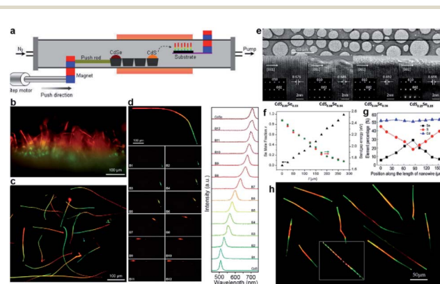
Fig. 2 Composition-graded \text{CdS}_{1-x}\text{Se}_x ( 0 \leq x \leq 1 ) ternary alloy nanowires. (a–f) \text{CdS}_{1-x}\text{Se}_x nanowires with a single composition gradient: (a) schematic diagram of source-moving thermal evaporation growth; (b) real-color optical photograph of (b) as-grown and (c) dispersed graded nanowires; (d) spatially resolved PL emission and corresponding spectra from a single graded nanowire; (e) TEM characterization; (f) position-dependent Se molar fractions and bandgaps. (g and h) \text{CdS}_{1-x}\text{Se}_x nanowire with symmetric dual composition gradients: (g) position-dependent molar fractions; (h) real-color optical photograph of dispersed nanowires. (a–f) Reproduced with permission. 11 Copyright 2011, American Chemical Society. (g and h) Reproduced with permission. 46 Copyright 2013, American Chemical Society.
