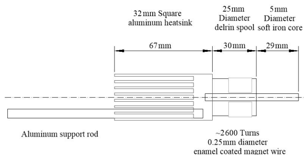
Figure 2 Schematic illustration of the electromagnetic device
