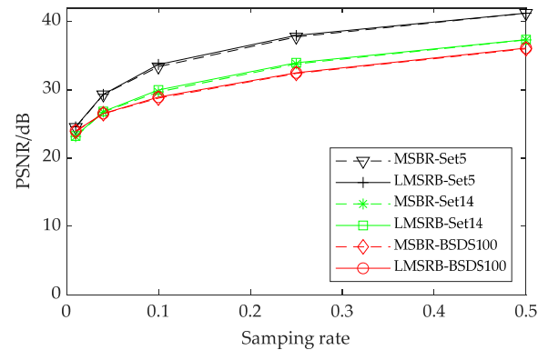
Figure 10. PSNR comparisons of two methods on three datasets at different sampling rates.
