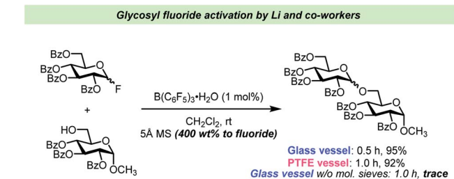
Scheme 5 Control experiments for vessel effect by Li and co-workers. 63 No experiment in PTFE vessel without mol. sieves was reported.
