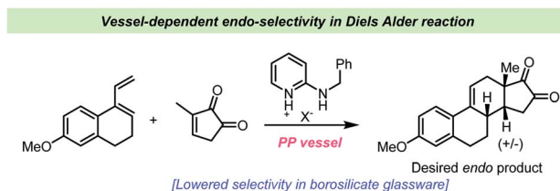
Scheme 12 Example of vessel-dependent selectivity in endo -selective Diels–Alder reactions reported by Schuster et al. 112
