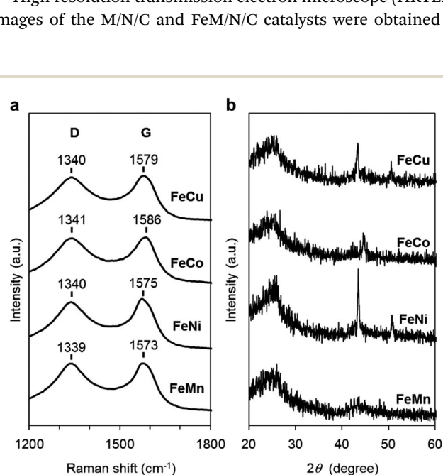
Fig. 4 Characterization of the FeM/N/C catalysts prepared from M(2NAPD) precursors. (a) Raman spectra and (b) XRD patterns of FeCu/2NAPD@VC, FeCo/2NAPD@VC, FeNi/2NAPD@VC, and FeMn/2NAPD@VC.
