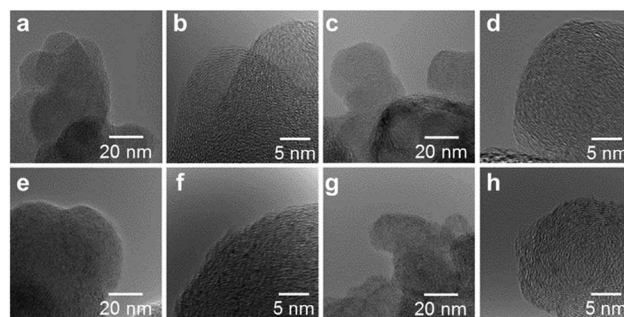
Fig. 6 HRTEM images of (a, b) FeCu/2NAPD@VC, (c, d) FeCo/2NAPD@VC, (e, f) FeNi/2NAPD@VC, and (g, h) FeMn/2NAPD@VC (magnification = 300k and 1000k). The metal content of each of the samples determined by EDS analysis with an electron probe of 25 nm in the area with 300k magnification is (a) Fe: 0.31 wt%, Cu: 0.18 wt%, (c) Fe: 0.33 wt%, Co: 0.16 wt%, (e) Fe: 0.33 wt%, Ni: 0.16 wt%, and (g) Fe: 0.40 wt%, Mn: 0.27 wt%.
