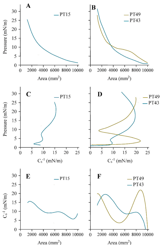
Fig. 3. Biophysical characteristics of meibum from donors with hematopoietic stem cell transplantation and dry-eye tear solution at 35 °C. Top row: pressure-area isotherms; middle row: reciprocal compressibility modulus ( C_s^{-1} ) as a function of surface pressure; and bottom row: C_s^{-1} as a function of surface area.
