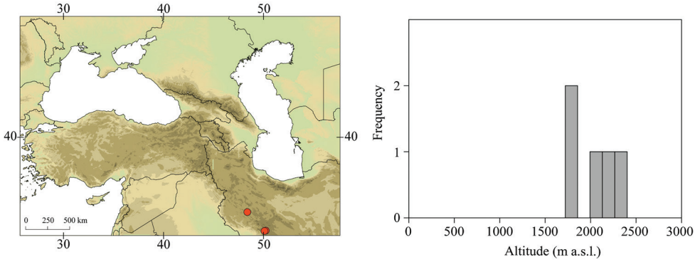
Figure 45. Geographical (left) and vertical (right) distribution of Epeorus (Caucasion) zagrosicus .
