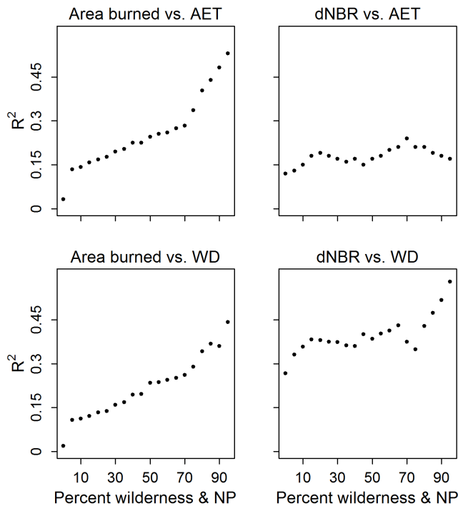
Figure 4. Strength of the relationship (R 2 for all models except the dNBR vs. AET model, which is evaluated with the r 2 ; see Methods) for all models as a function of increasing percentage of wilderness and national park in each hexel. doi:10.1371/journal.pone.0099699.g004
