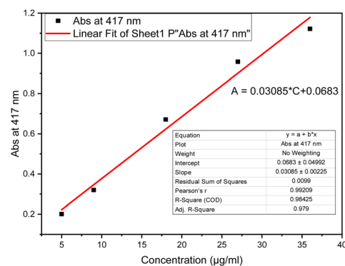
Fig. 3 UV-Vis spectra and calibration curves of TP as gallic acid (a) and TA as atropine (b).
