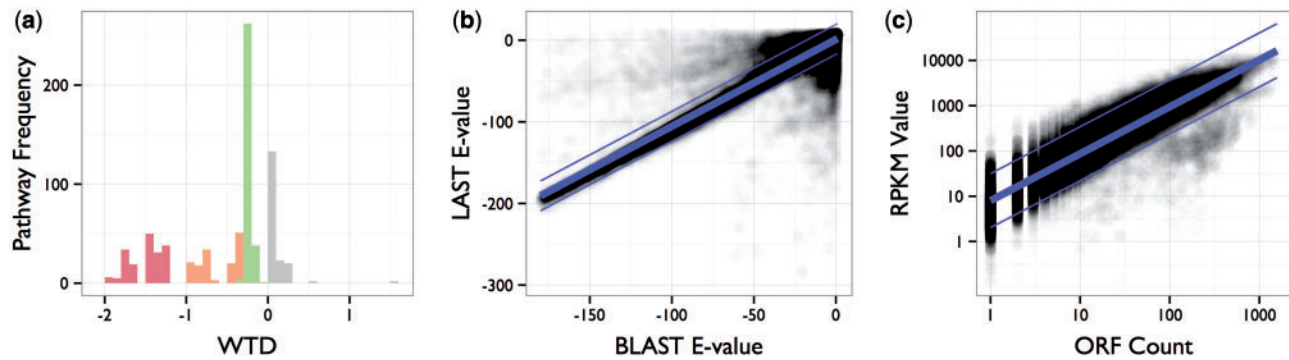
Fig. 1. Quantitative functional and taxonomic improvements. (a) WTD provides a measure of taxonomic agreement between observed RefSeq Lowest common ancestor (LCA) taxonomy and the expected taxonomic range of predicted MetaCyc pathways, separated into the ‘High’ (Red), ‘Medium’ (Orange) and ‘Low’ (Green) taxonomic hazard classes based on negative quartile order statistics. Positive distances represent taxa found within a pathways expected taxonomic range and so have a hazard class of ‘None’ (Grey). (b) The LAST and BLAST homology search algorithms are highly correlated in terms of E-value ( R^2 = 0.887 , P < 0.01 ). (c) ORF Count and the RPKM measure show a linear relationship ( R^2 = 0.816 , P < 0.01 ). Ninety percent of prediction intervals, displayed as a pair of thin blue lines about the fitted line, capture \sim 96.7 and 91.3\% of observed points in (b) and (c) , respectively. Analysis code can be found in the Supplementary information
