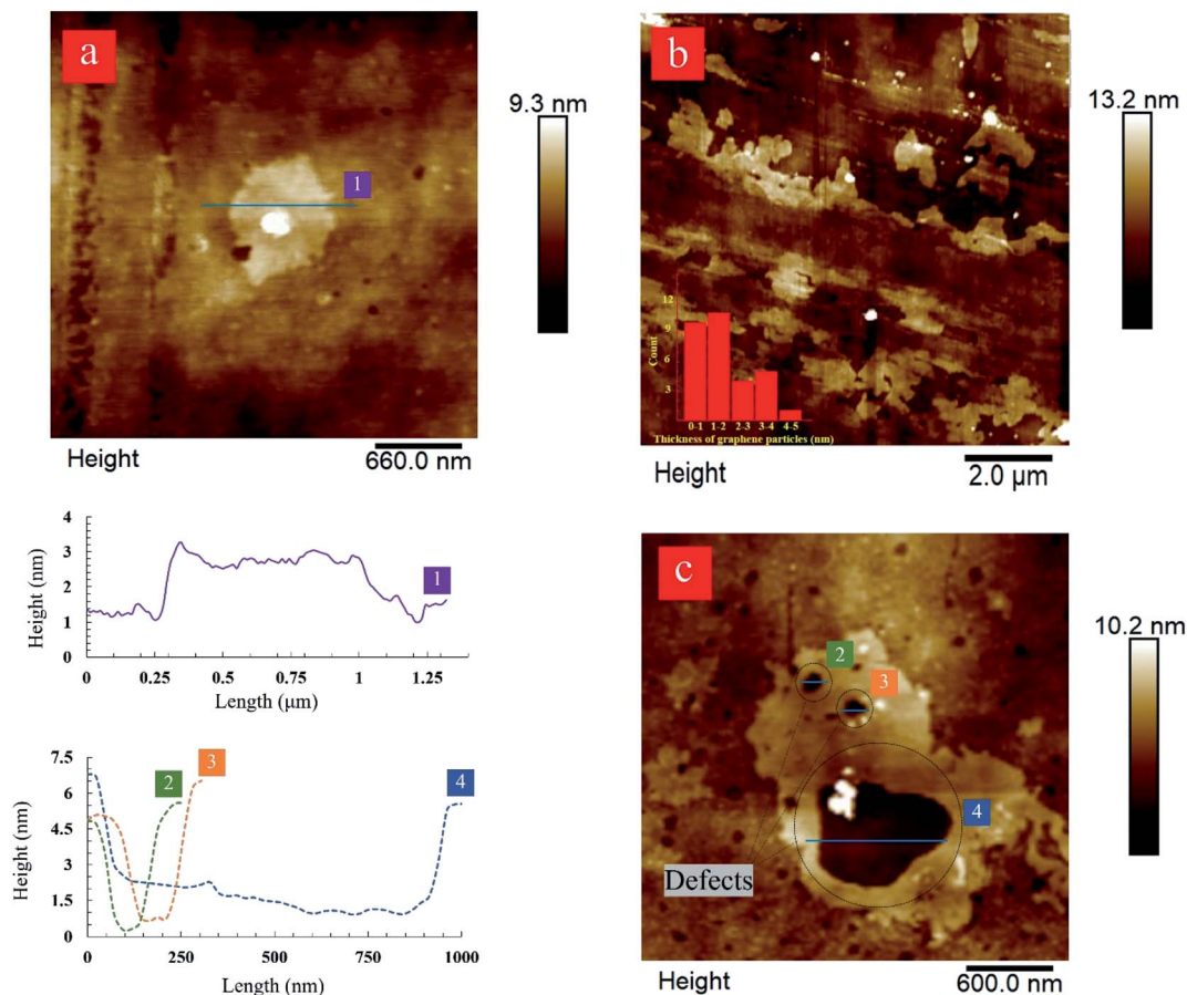
Fig. 6 AFM images of monolayer and few layers of graphene sheets. (a) A graphene sheet with a thickness about \sim 1 nm after 80-cycles, (b) the exfoliated graphene nanosheets large in lateral size after 60-cycles of treatment, and (c) a graphene sheet with defects, which were formed by exposure to excessive bubble collapse after 60-cycles.
